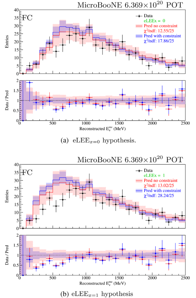
FIG. 26. Event distributions of FC \nu_e CC candidates as a function of reconstructed E_\nu . (a) An e\text{LEE}_{x=0} hypothesis and (b) an e\text{LEE}_{x=1} hypothesis are assumed in MC prediction and uncertainty calculation, respectively. Black points are from data measurements. Red (blue) histograms and error bands are for MC prediction before (after) constraint from the other six channels.
