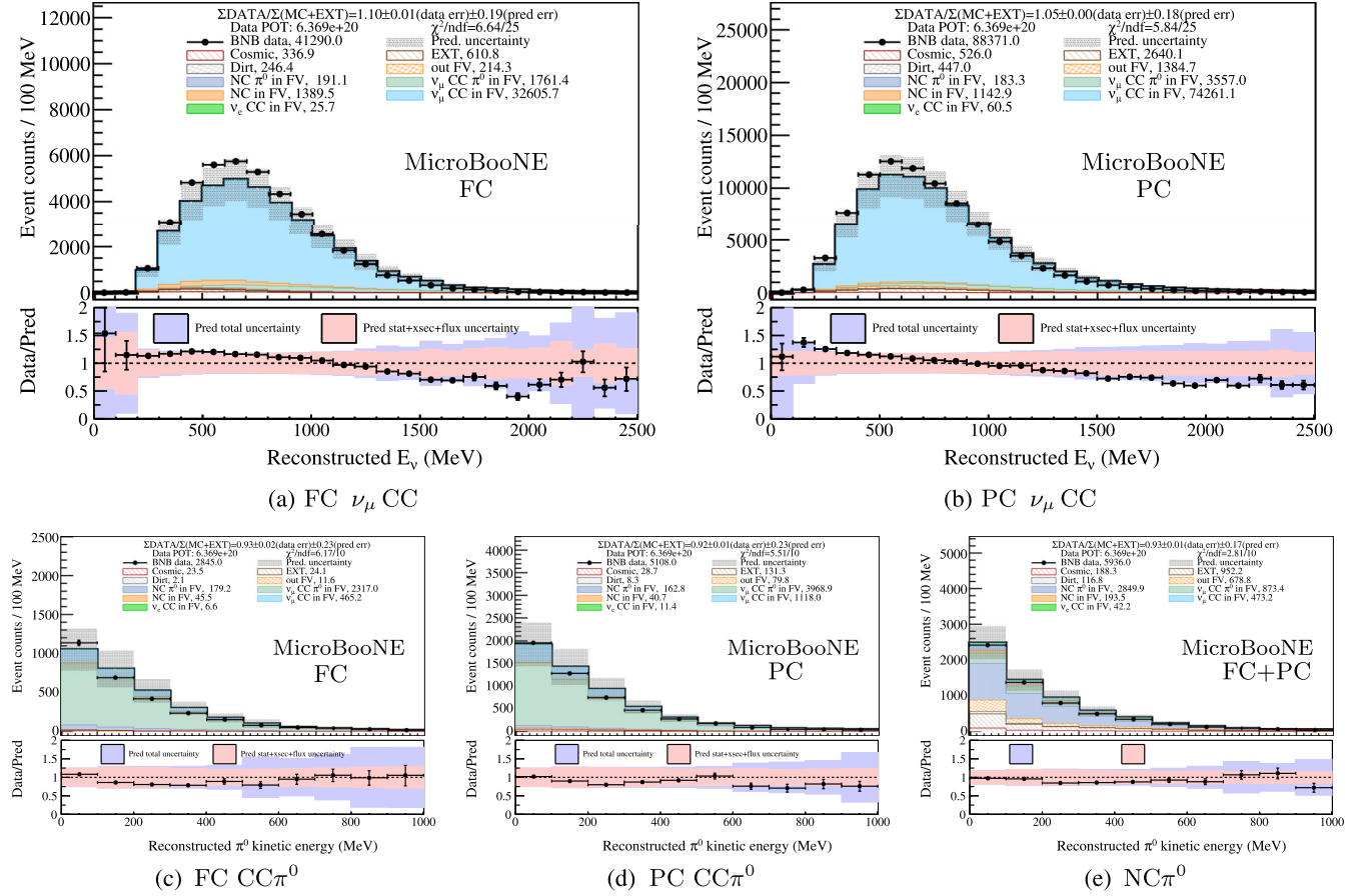
FIG. 21. Event distributions of FC \nu_\mu CC, PC \nu_\mu CC, FC CC\pi^0 , PC CC\pi^0 , and NC \pi^0 in (a)–(e), respectively. These five selections serve as constraints to reduce the systematic uncertainties in searching for eLEE, thus maximizing the physics sensitivity. The breakdown of each component for different final states for both signal and background events is shown in the legend. The bottom subpanels present the data-to-prediction ratios as well as the statistical and systematic uncertainties. The pink band includes the statistical, cross-section, and flux uncertainties. The purple band corresponds to the full uncertainty with an addition of detector systematic uncertainty.
