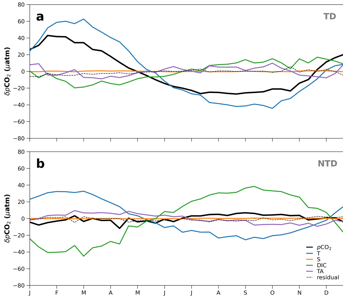
Figure 3. Decomposition of the p\text{CO}_2 seasonal cycle (black), expressed as a deviation from the annual mean, into components associated with variations in surface temperature (blue), salinity (orange), DIC (green), and TA (purple). The components are calculated from the float climatologies for the (a) thermal and (b) non-thermal regimes using Equations 1–5. Residuals are plotted as black dashed lines in each panel.
