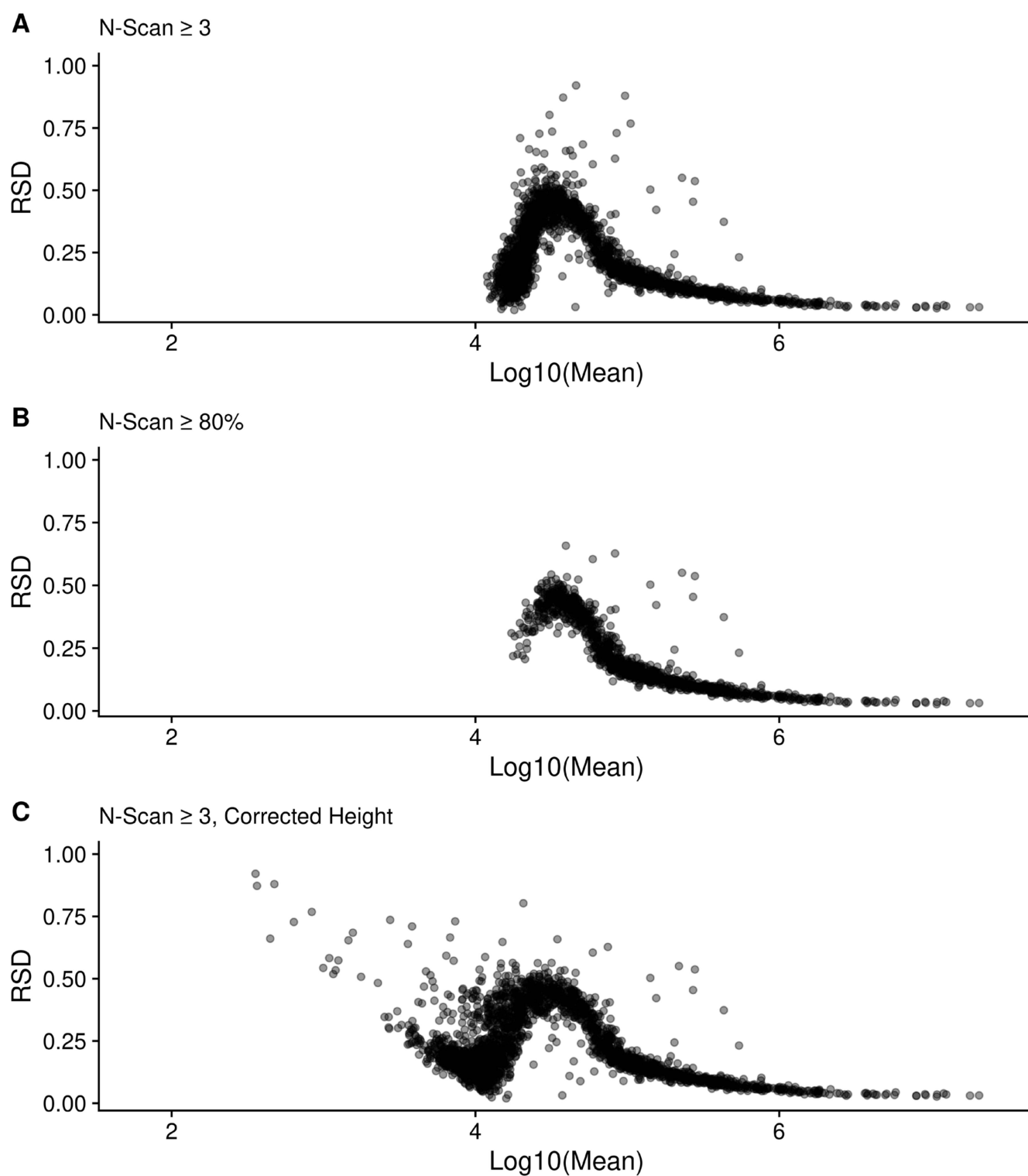
Figure 12. RSD as a function of the log-mean peak intensity for the filtersd method peaks from the 97lipid sample. (A) shows all peaks in at least three scans using raw height; (B) shows peaks that were present in at least 80% of the scans; and (C) shows all peaks in at least three scans using the corrected height.
