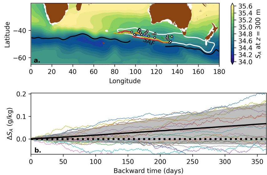
Figure 3. (a) Examples of the backwards trajectories of 20 Lagrangian particles following the geostrophic flow in the Indian Ocean (90°E–135°E), and (b), mean (black line) and standard deviation (shading) of the annual-mean absolute salinity change ( \Delta S_A = S_A(t) - S_A(t=0) ) along backward trajectories. In (a), filled contours represent the climatological mean S_A at 300 m; black contour, the sub-Antarctic front (SAF); white contour, the seasonal maximum MLD of 500 m, and, white dots, the particles' initial positions.
