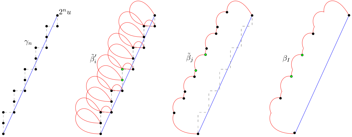
Figure 3: Construction of “nice paths”. (The “lifting” step is omitted here to aid visualization).
