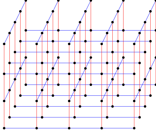
Figure 2: A portion of the Cayley graph of \langle \rho \rangle \ltimes \mathbb{Z}[i] with respect to the generating set \{\rho, 1 + 0i\} . Edges labeled by \rho are red, while edges labeled by 1 + 0i are blue.
