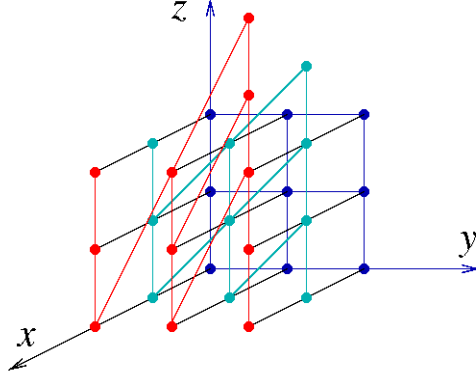
Figure 1: A portion of the Cayley graph of H(\mathbb{Z}) with respect to the generating set \{X, Y, Z\} . Source: Wikipedia; image by Gabor Pete. Colors are for visual contrast only.
