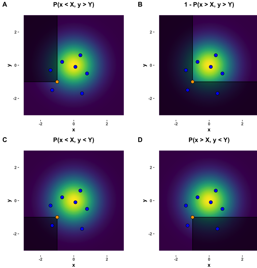
Figure 2: Four ways (3 independent) of defining the cumulative distribution for a given point in 2-D. Here, the orange point (X, Y) is chosen as the origin; the density of observations may be integrated as \mathbb{P}(x < X, y > Y) (A); \mathbb{P}(x < X \cup y < Y) (B); \mathbb{P}(x < X, y < Y) (C); \mathbb{P}(x > X, y < Y) (D).
