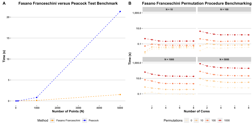
Figure 5: Computational efficiency benchmarks. A: Runtime of the Fasano–Franceschini test relative to the Peacock test at four different sample sizes ( n = 10, 100, 1000, 5000 ). Points represent the average of 10 benchmark runs. B: Runtime of the Fasano–Franceschini permutation procedure for various sample sizes ( n = 10, 100, 1000, 5000 ) as a function of the number of cores used. Within each panel, lines are colored by the number of permuted iterations (no permutation, 10, 100, 1000). Points represent the average of 10 benchmark runs. Note the logarithmic y -axis in (B).
