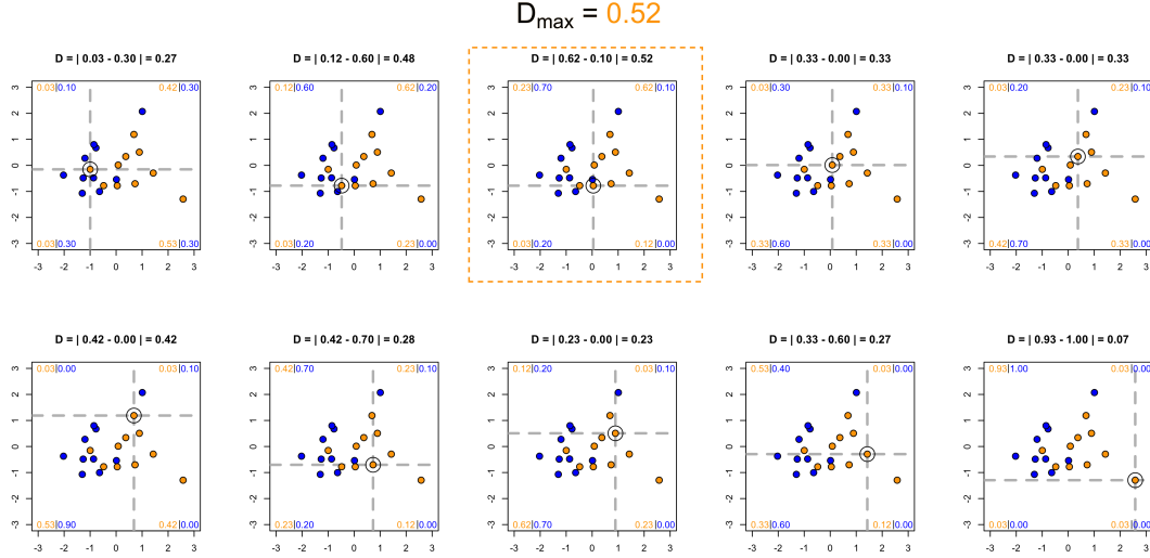
Figure 3: Illustration of the Fasano–Franceschini algorithmic search for the maximal difference ( D_{FF,1} ) between sample 2-D eCDFs. Looping through each point in the sampled data to define a unique origin (grey dotted line), the fraction of orange and blue points in each quadrant are computed (plot corners). For each origin, the quadrant which maximizes the absolute difference in the integrated probabilities is indicated. The origin which maximizes the overall absolute difference in the integrated probabilities between samples is highlighted by the orange box.
