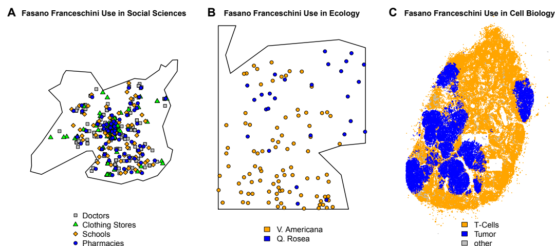
Figure 4: Example application settings for the Fasano-Franceschini test. A: Geographic locations of four distinct facilities in the municipality of Rennes, France (Floch et al., 2018). B: Geographic location of tree species in the plot 16 field station of the Paracou Forest, French Guiana (Marcon et al., 2015). C: Immunohistochemistry stained tumor-infiltrated lymph node cross section, with tumor and T-cells colored in blue and orange respectively (Set, 2010).
