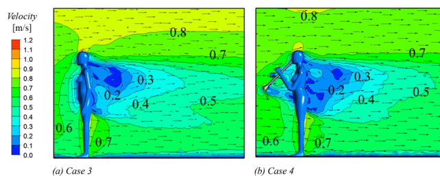
Figure 17. Flow field in the vertical section through the middle of the musician's body in an outdoor environment.
