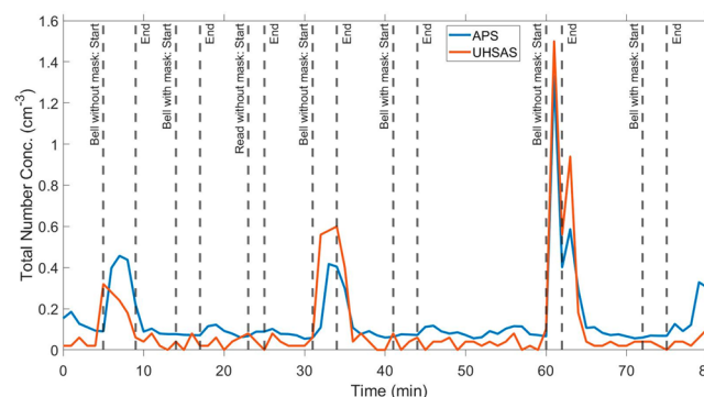
Figure 11. UHSAS and APS total number concentration for clarinet player for the overlapping size range common between the two instruments, \sim 540 – 980 \text{ nm} . Time series of total concentrations played on the clarinet.
