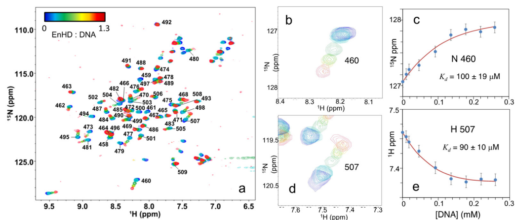
Figure 7. (a) Series of ^1\text{H} - ^{15}\text{N} -HSQC NMR spectra of 3nHD (at 0.2 mM in 20 mM acetate, pH 4, NaCl 0.3 M and T = 298\text{ K} ) at different concentrations of cognate DNA up to a 1:1.3 ratio of enHD to DNA. Numbered labels indicate the residue assignment in reference to the full Engrailed sequence. The color bar on the top left indicates the particular enHD to DNA ratio for each spectrum. (b) Detail of the spectral region corresponding to residue A460 (colors as in (a)). (c) ^{15}\text{N} chemical shift of residue A460 as a function of cognate DNA concentration fitted to an equilibrium binding equilibrium (red line). (d) Detail of the spectral region corresponding to residue A507 (colors as in (a)). (e) ^1\text{H} chemical shift of residue A507 as a function of cognate DNA concentration fitted to an equilibrium binding process (red line, Equations (1) and (2)).
