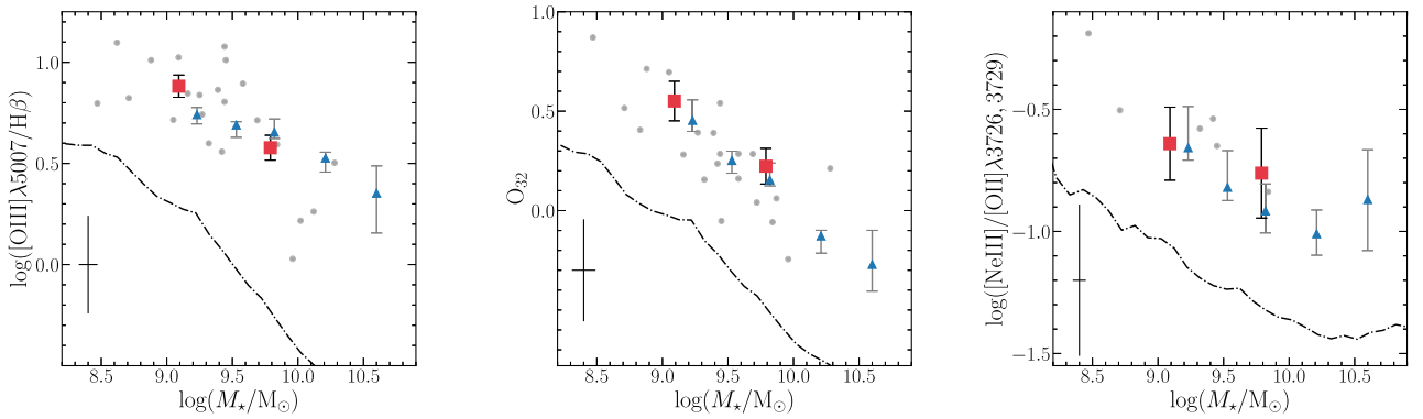
Figure 7. Dust-corrected emission line ratios versus M_* for galaxies at z \approx 3.4 and z \approx 0 . Each panel shows one of the three emission-line ratios used to determine Z_g in this paper (see Section 3). From left to right, these line ratios are [O\text{III}]/H\beta , O_{32} , and [Ne\text{III}]/[O\text{II}] . The red squares show the low- M_* and high- M_* NIRVANDELS stacks (see also Fig. 5) and the grey circles show the individual NIRVANDELS galaxies with the necessary line detections. The median error bar on the individual detections is shown in the bottom left-hand corner. The blue triangular data points show stacked measurements from the z \approx 3.3 MOSDEF sample presented in Sanders et al. (2020a). The dot-dashed lines represent the running medians for z \approx 0 galaxies from the SDSS sample of Andrews & Martini (2013). These z \approx 0 line ratios have been corrected, where possible, for diffuse ionized gas (DIG) contamination that can bias line flux measurements in local galaxies [see the text and Sanders et al. (2020a) for further details].
