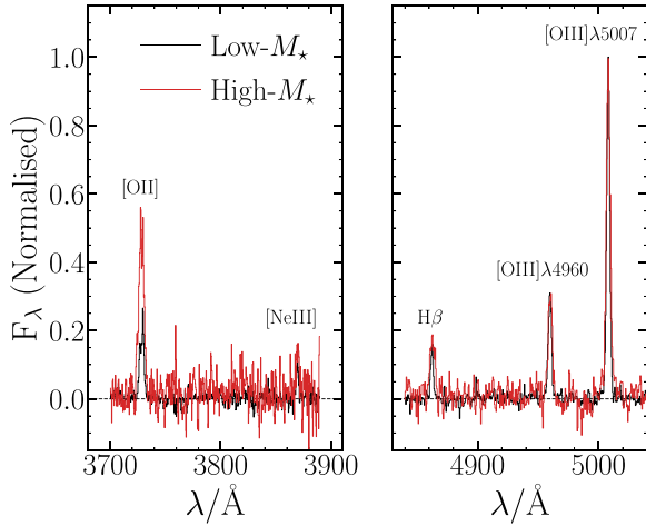
Figure 5. Portions of the MOSFIRE composite spectra in the H band (left) and K band (right), covering the [O II], [Ne III], H\beta , and [O III] \lambda 5007 nebular emission lines. The low- M_* composite is shown in black and the high- M_* stack in red. Both composites have been normalized by the peak [O III] \lambda 5007 flux of the low- M_* composite spectrum.
