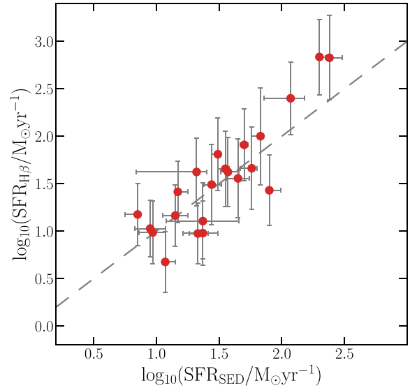
Figure 1. A comparison between star formation rate derived from the photometry and the dust-corrected \text{H } \beta line flux for the 22 galaxies in our sample with a >2\sigma detection of the \text{H } \beta line. The grey dashed line shows the one-to-one relationship.
