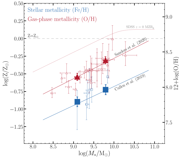
Figure 8. The mass–metallicity relation for stars ( Z_* , blue squares) and nebular gas ( Z_g , red triangles) within the NIRVANDELS galaxies at z \approx 3.4 . The small open data points show Z_* and Z_g for individual galaxies, and the large filled data points show the low- M_* and high- M_* stacks. The blue and red solid lines show, respectively, previous determinations of MZR_* and MZR_g at z \approx 3.4 from Cullen et al. (2019) and Sanders et al. (2020a). The Cullen et al. (2019) MZR_* has been re-calculated to account for shifts in M_* as described in the text (Section 4.1.2). The grey dotted line shows the DIG-corrected MZR_g at z \approx 0 from Sanders et al. (2020a), and the horizontal dashed grey line indicates the value of solar metallicity on the y-axis. On the right-hand side of the y-axis, we show the value of \log(\text{O/H}) + 12 for the Z_g data (the conversion is given by 12 + \log(\text{O/H}) = \log(Z_g/Z_\odot) + 8.69 ).
