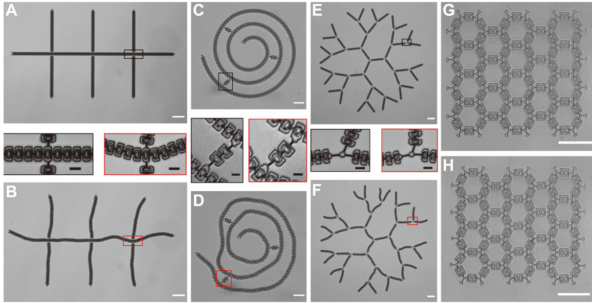
Fig. 2. Pre- and post-release transmission brightfield microscopy images of fabricated polyolithomers immersed in a release solution-dispersion (RSD). Symmetric branched PLM: (A) before release and (B) 30 h after release. 3-Bridged chiral(-) spiral PLM: (C) before and (D) 30 h after release. 3-2-2-2 Dendrimer PLM: (E) before and (F) 30 h after release. Quasi-2D honeycomb mesh PLM: (G) before and (H) 30 h after release. Corresponding zoomed images (between parts A and B, C and D, and E and F) show branching points: pre-release (black boxes) and post-release (red boxes). Brownian excitations cause fluctuations in conformations of post-release PLMs. Scale bars: 50 \mu\text{m} (white), 10 \mu\text{m} (black).
