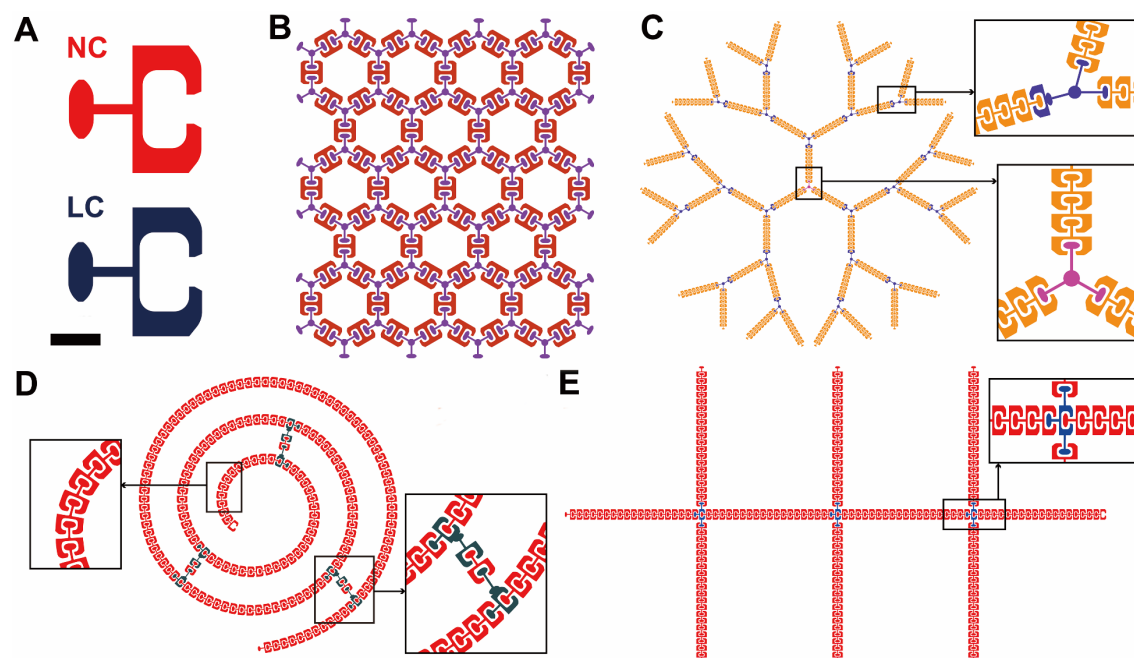
Fig. 1. Designs of lithographic monomers (lithomers, LMs) and sterically bonded lock-and-key polyolithomers (PLMs). (A) Basic LMs designed to have convex heads and tails with concave cavities: normal cavity (NC; red, top); larger cavity (LC, dark blue, bottom). Internal cavity lengths are 4.5 \mu\text{m} for NC and 5.0 \mu\text{m} for LC. Scale bar: 5 \mu\text{m} in wafer scale. (B) Quasi-2D honeycomb mesh PLM composed of di-cavity LMs (dark red) and tri-head LMs (purple). (C) 3-2-2-2 dendrimer PLM. Insets: mono-cavity, di-head branched LM (blue, top box) and tri-head LM (magenta, bottom box). (D) 3-Bridged chiral(-) spiral PLM. The LMs here have intrinsic curvatures that vary along the spiral. Insets: LMs designed to have non-zero intrinsic curvature (left box); Crosslinking LMs (right box). (E) Symmetric branched PLM having 3 pairs of symmetric side chains off a central backbone. Inset (box, arrow): detail showing multi-headed branching LM (blue) at a branching point.
