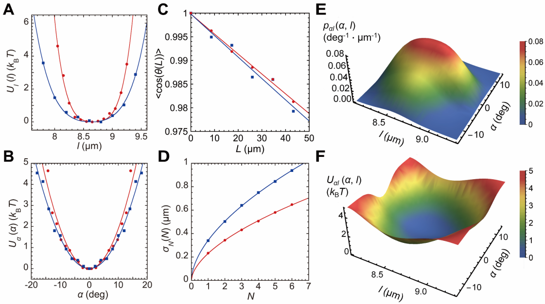
Fig. 4. Equilibrium bond characteristics of PLM NCS and PLM LCS : designer bond extensibility and semi-flexibility. (A) Extracted potential of interparticle centroid spacing, U_l(l) , between adjacent LMs, assuming Boltzmann statistics, irrespective of bond angle \alpha : PLM NC (red circles) and PLM LC (blue squares). Solid lines: fits to quartic potentials for NC-type (red, R^2 = 0.993 ) and LC-type (blue, R^2 = 0.998 ). Fitted most probable spacing l_0 between LMs for both NC and LC types of PLMs are nearly the same: l_0 \approx 8.65 \mu\text{m} . (B) Extracted potential of bond angle, U_\alpha(\alpha) , assuming Boltzmann statistics and U_\alpha even in \alpha , irrespective of l . Solid lines: fits to quadratic potentials for NC-type (red, R^2 = 0.94 ) and LC-type (blue, R^2 = 0.98 ). (C) Persistence length L_p is obtained by fitting observations of \langle \cos(\theta) \rangle (symbols same as in part a) as a function of length along the contour, L , to \exp(-L/L_p) : NC-type (red line, R^2 = 0.994 ); LC-type (blue line, R^2 = 0.966 ). (D) Standard deviation \sigma_N of spacing between N LMs along a PLM chain (symbols same as in part A). Fits to power law functions: NC-type (red line, R^2 = 0.9997 ); LC-type (blue line, R^2 = 0.9998 ). Surface plots for NC-type PLMs: (E) 2D probability density function, p_{\alpha l}(\alpha, l) , assuming even symmetry for \alpha , and (F) extracted 2D inter-LM potential U_{\alpha l}(\alpha, l) from part E assuming Boltzmann statistics.
