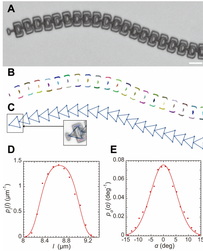
Fig. 3. Particle tracking and statistical properties of linear chains of PLMs obtained from arms of branched PLMs. (A) Transmission micrograph of an arm of NC-type LMs (grayscale from RGB color). Scale bar: 10 \mu\text{m} . (B) Extracted morphological components of part A, yielding head and tail sub-particle features (colored regions). Each head produces one colored region; each tail produces two colored regions, one on each side of the cavity. (C) Triangles represent extracted positions and orientations of LMs from centroids of morphological components in part B. Inset: overlay of (A-C) onto one monomer. (D) Observed probability density of interparticle ( i.e. inter-LM) centroid spacing, l , defined as the distance between the centers of two adjacent triangles, of \text{PLM}_{\text{NCS}} irrespective of the inter-LM bond angle \alpha . Fit: quartic potential in a Boltzmann distribution (line, see text, R^2 = 0.98 ). (E) Observed probability density of \alpha , defined by the relative orientation between two adjacent triangles of \text{PLM}_{\text{NCS}} , assuming even symmetry about \alpha = 0 and irrespective of l . Fit: quadratic potential in a Boltzmann distribution (line, see text, R^2 = 0.98 ).
