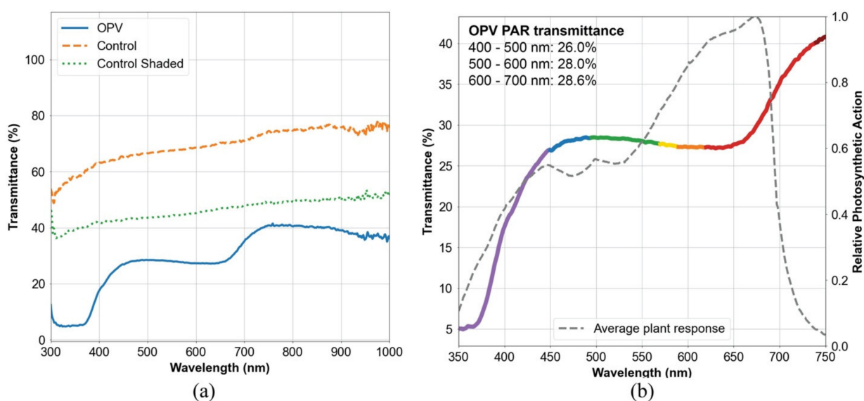
Figure 7. Canopy-level lighting quality in OPV and Control sections: (a) comparing OPV and Control sections with and without a shade net installed, measured at midday with a clear sky; (b) comparing the light transmittance in the PAR region in the OPV section to the relative photosynthetic action (efficiency), shown in the dashed gray line, which was adapted from McCree [19].
