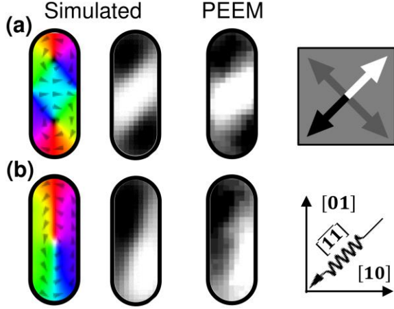
FIG. 2. (a, b) Simulated (left and center) and XMCD-PEEM (right) images of the double (a) and single (b) vortex spin textures. The colored regions in the vector field map (left) represent the in-plane component of the magnetization (also indicated by the arrows). The simulated XMCD images in the center have been processed to reflect both the experimental geometry and resolution (see text for processing details). The contrast in both PEEM and simulated XMCD images were enhanced for visual clarity. Schematics of the experimental geometry and associated magnetic contrast for both PEEM and simulated images are shown in the far right.
