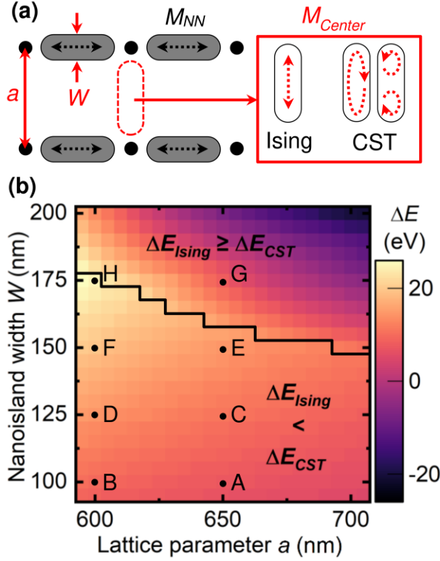
FIG. 3. (a) Schematic of the five-island unit simulated to determine the relative energies when the red center nanoisland takes on an Ising or CST state (i.e., single or double vortex). Each nearest neighbor magnetization ( M_{NN} ) can have two possible orientations. (b) Minimum energy surface calculated relative to a configuration with two Type I vertices, E_{Dual\ I} (equation 2). The black line separates the regions where the minimum \Delta E is associated with an Ising M_{Center} ( \Delta E_{Ising} < \Delta E_{CST} ) or a CST M_{Center} ( \Delta E_{Ising} \geq \Delta E_{CST} ). Letters correspond to the ASI configurations listed in Table I.
