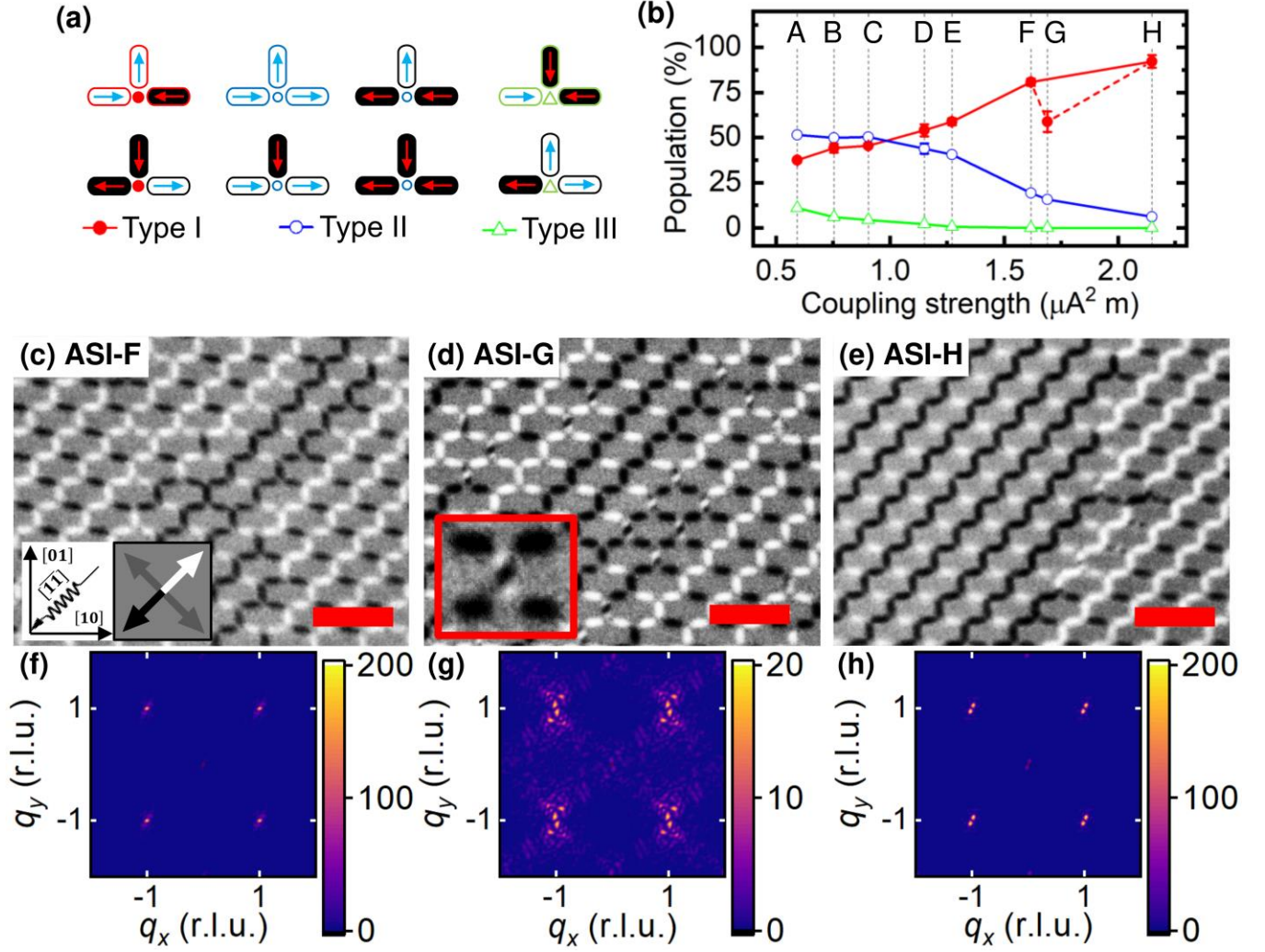
FIG. 1. (a) Schematic of the eight possible Ising-like moment configurations at a three-nanoisland vertex. Type I, II, and III vertices are designated as red solid circles, blue open circles, and green triangles, respectively. (b) Average vertex population for ASIs A-H plotted as a function of coupling strength, J . Each error bar correspond to the standard deviation between 2-4 unique XMCD-PEEM images of the ASIs. In ASI-G, the Ising model breaks down as the magnetic configuration of 9\% \pm 2\% of the nanoislands cannot be classified as single domains, causing a deviation in the Type I population trend as indicated by the dashed line. (c-e) XMCD-PEEM images and (f-h) corresponding MSF calculations of ASI-F (c, f), ASI-G (d, g), and ASI-H (e, h), respectively. The experimental geometry and associated magnetic contrasts are schematically shown on the legends. Inset in (d) shows a zoom-in image of a multidomain nanoisland with contrast enhanced for visual clarity. MSFs were calculated by assuming an Ising model where CST islands possess zero net moment. Red scale bars are 2 \mu\text{m} . r.l.u., reciprocal lattice units, based on a square ASI lattice.
