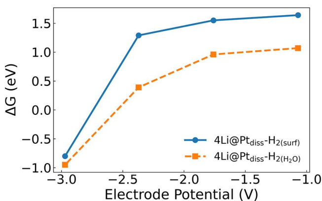
Figure 5. Free energies of the discharge reactions (1) and (2) as a function of applied bias potential for the 4Li@Pt diss dissolution state shown in Figure 4d. Both initial and final atomic configurations for each reaction were optimized at a given electrode potential after being extracted from AIMD trajectories.
