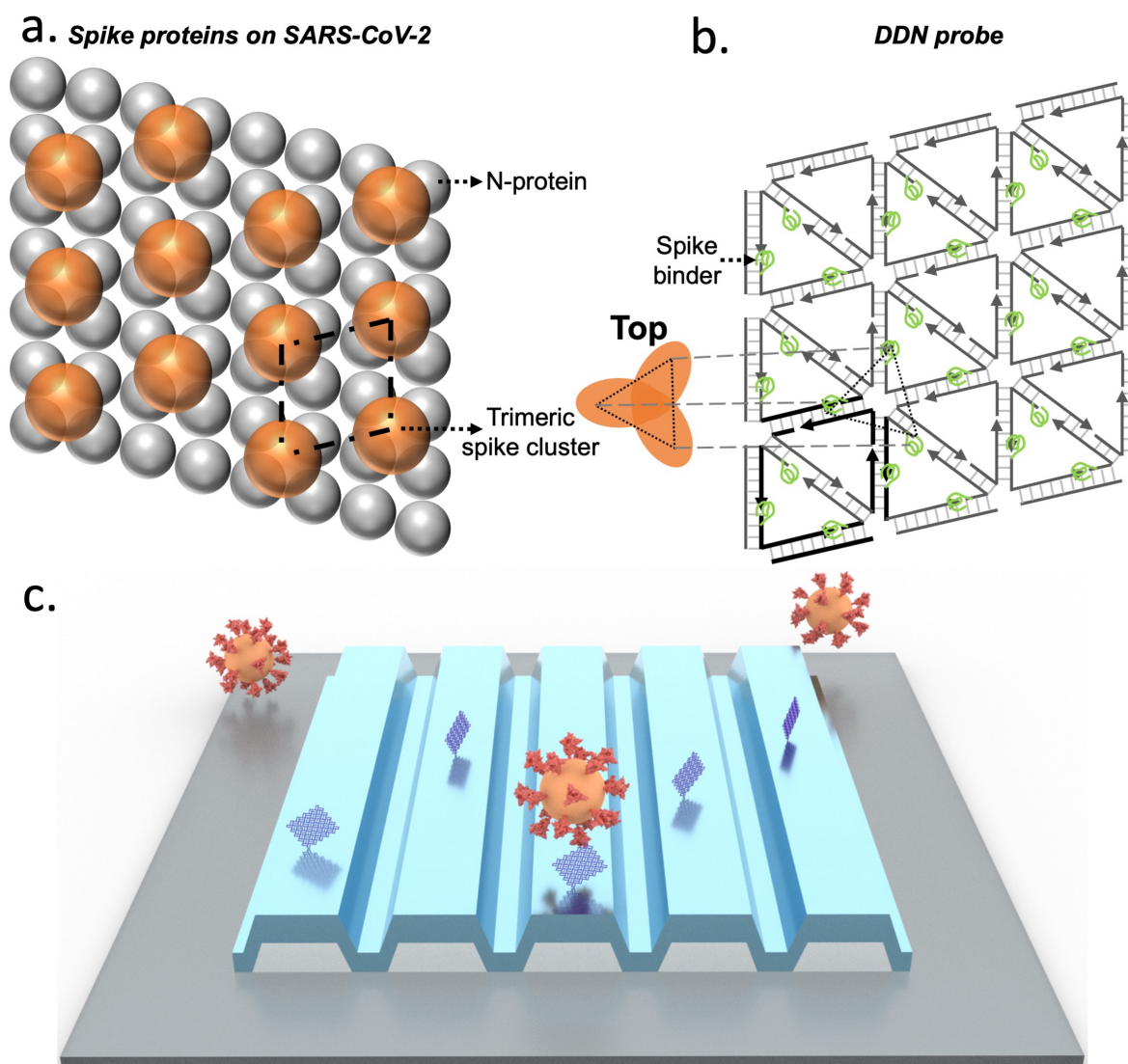
Figure 4. SARS-CoV-2 virion sensing using PRISM. (a) Spatial arrangement of SARS trimeric spike proteins and nucleoproteins (N). (b) The DDN probe can be designed and synthesized to match the pattern and spacing of trimeric spike clusters. 3' end of each DNA oligo is indicated by an arrow. Three spike-targeting binders will be placed on each vertex. (c) The PC incorporates active sensing regions with DDN probes attached to the active region for selective capture of SARS-CoV-2 virions.
