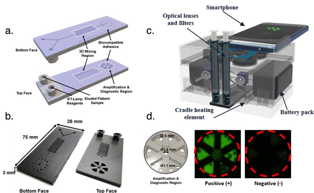
Figure 7. AM cartridge and portable detection cradle. (a) Labeled cartridge schematic. The inlets mate with Luer lock syringes to deliver the reagents and samples to the rest of the chip. (b) Cartridge images (c) Assembled view of POC cradle with smartphone and optical components. (d) Detailed view of detection region and images of positive and negative sample tests after 40 minutes. a, b, extracted from 27 .
