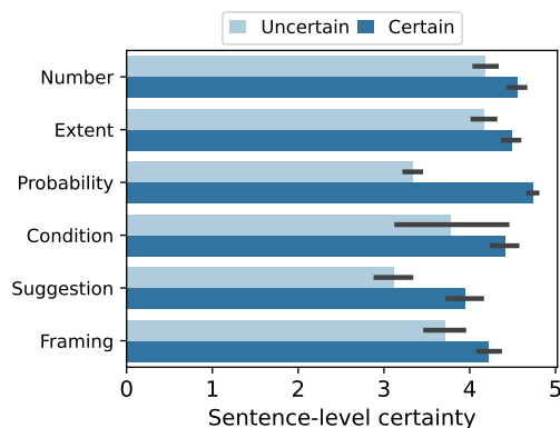
Figure 3: Relative sentence-level certainty when each aspect is certain/uncertain. the overall certainty of scientific findings are majorly affected by PROBABILITY and SUGGESTION, while are less affected by other aspects like NUMBER and EXTENT
