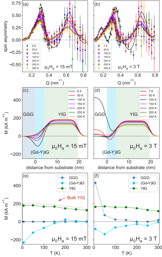
FIG. 2. PNR spin asymmetry [(a), (b)], magnetization profiles determined from model fitting [(c), (d)], and resulting M vs T measured for \mu_0 H = 15 mT (left) and \mu_0 H = 3 T (right). The three magnetic components of the sample are shown in background shading in panels (c) and (d), and their M separately plotted in (e) and (f). We provide bulk values of M(T) for YIG for comparison in panel (e).
