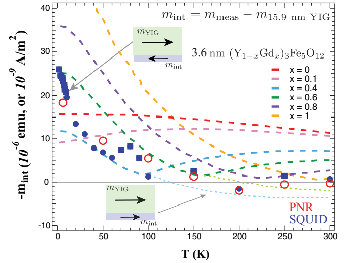
FIG. 7. Estimated moment of the (Gd-Y)IG interface layer, -m_{\text{int}} vs T from SQUID magnetometry (blue symbols), and PNR (red circle) compared to bulk values of (\text{Gd}_x\text{Y}_{1-x})_3\text{Fe}_5\text{O}_{12} for various x (dashed lines). For the x = 0.4 and x = 0.6 mixed garnets we also show the moment with reversed sign above T_{\text{comp}} , which roughly brackets the measured -m_{\text{int}} from both PNR and SQUID at high T . At low T , -m_{\text{int}} again falls roughly between the values for x = 0.4 and x = 0.6 , suggesting that the interface layer has a high Gd content, though is most likely not purely bulk-like GdIG.
