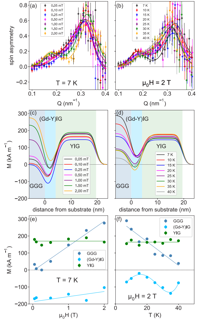
FIG. 3. PNR spin asymmetry [(a),(b)], modeled magnetization profiles [(c),(d)], and resulting M vs \mu_0 H at fixed T = 7 K (e) and M vs T at fixed \mu_0 H = 2 T (f). Solid lines in (e) and (f) are guides to the eye. Possible nonmonotonic behavior of the (Gd-Y)IG layer could result from frustrated domains in this interfacial layer. Note however that the negative M at all \mu_0 H for the (Gd-Y)IG indicates very strong antiferromagnetic exchange at the interface.
