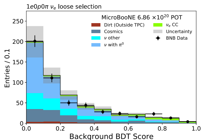
FIG. 6. 1e0p0\pi selection BDT response. Background events are predicted to peak at low BDT scores and electron neutrino events at high BDT scores. In the final selection, events with BDT scores above 0.72 are retained. Gray bands denote the systematic uncertainty on the prediction.
