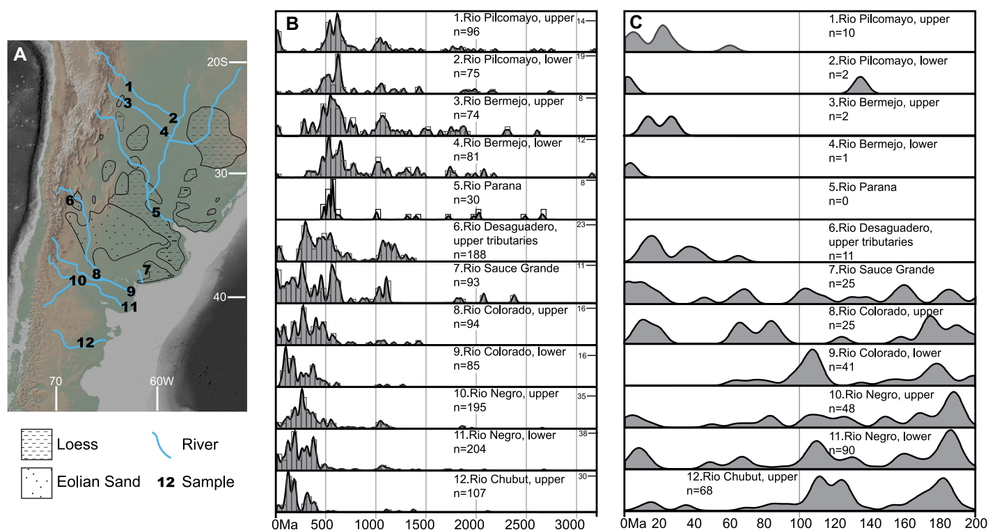
Figure 4. Existing detrital-zircon data from modern rivers in the Central and Southern Andes. (A) Digital elevation model image of southern South America with rivers, eolian deposits, and sample locations. (B and C) Detrital zircon data from modern rivers. (B) Zircon age distribution of samples for grains with ages between 0 and 3200 Ma. Kernel density estimates (KDE) and histogram are shown. (C) KDE results of detrital zircons with ages <200 Ma. Sources for data: 1–4 and 7–12 Pepper et al. (2016; original samples: CA01, CA02, CA03, CA04, SA06, SA07, SA08, SA09, SA11, and SA12 combined, SA15); 5 Rino et al. (2008; original samples: Para); 6 Capaldi et al. (2017; original combined samples RBMJ01 and RSJN03).
