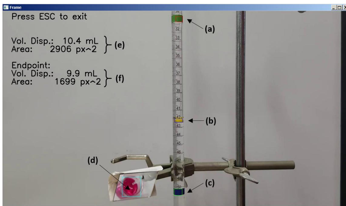
Figure 2. Screenshot of the CV script window: (a) top mark; (b) titrant level mark; (c) bottom mark; (d) mirror image of the analyte solution; (e) interactive and (f) endpoint of titration data on volume of the dispensed titrant solution and area of the fuchsia (pink) spot. The script automatically tracks marks and the fuchsia spot outlining them with rectangles. The video recording is available at: https://youtu.be/QBwOgbi6VbU&t=4m16s
