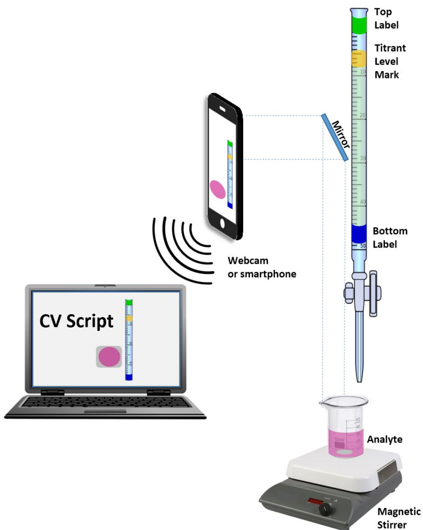
Figure 1. Experimental setup: a standard burette is labeled with top and bottom label marks to indicate minimal and maximal volume of the titrant. A free-floating bead is used to indicate the level of titrant. A top-view image of the analyte solution is projected to the webcam/smartphone by the mirror. The CV script installed on the computer performs automatic analysis of the titration experiment progress.
