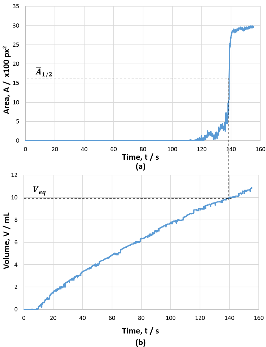
Figure 7. (a) Area ( A ) of the fuchsia spot and volume ( V ) are measured by the CV script. (b) The equivalence volume ( V_{eq} ) is determined automatically when the area of the fuchsia spot is reached half of its averaged maximal value ( \bar{A}_{1/2} ).
