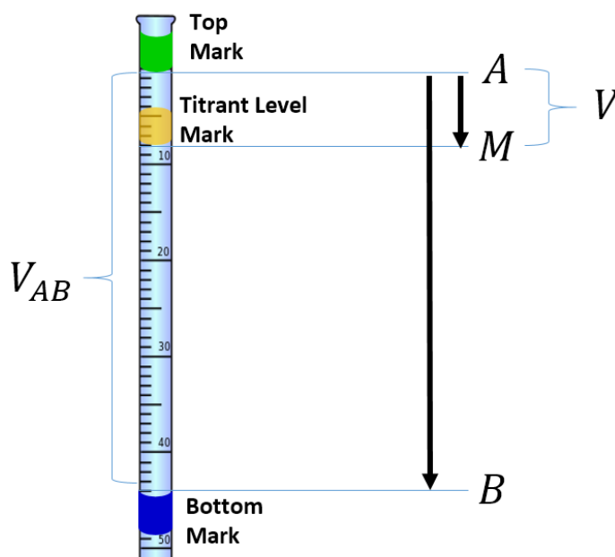
Figure 4. The volume of the titrant solution is determined based on coordinates of vectors \overrightarrow{AB} and \overrightarrow{AM} (see explanation in the text)
