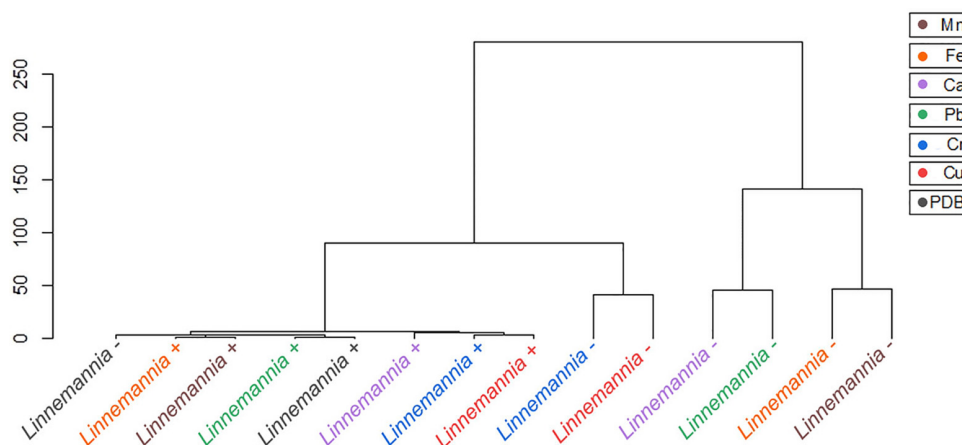
FIGURE 9 | Hierarchical cluster analysis of the ATR-FTIR spectra of the Linnemannia + and Linnemannia -. The Euclidean method was used to determine the distance between the different samples.
