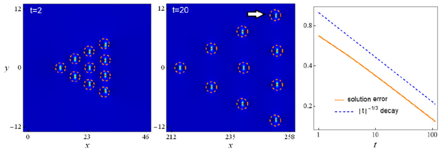
Fig. 5 Verification of the error decay rate in Eq. (35) of Theorem 2 for the example of Fig. 4. The left and middle panels show density plots of true solutions, together with predicted locations of fundamental lumps marked by dashed circles, at t = 2 and 20 , respectively. The right panel shows the decay rate of error versus t for the lump marked by a white arrow in mid-panel (the |t|^{-1/3} decay is also plotted for comparison)
