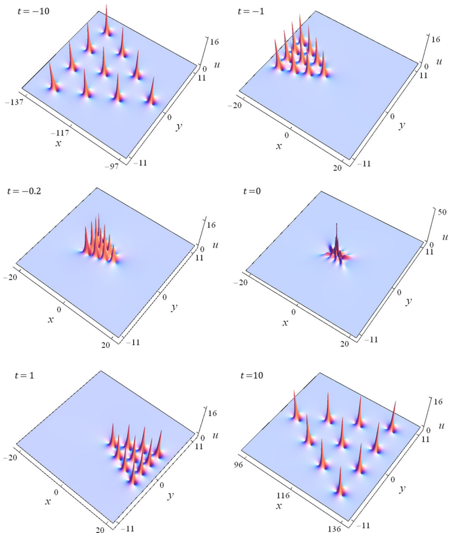
Fig. 4 True solution u_{\Lambda}(x, y, t) with \Lambda = (1, 3, 5, 7) and \mathbf{a} = (0, 0, 0, 0, 0, 0, 0) at various time values shown inside the panels. In all panels, lengths of the x intervals are the same, but the intervals are changing since the wave ensemble is moving along the x direction at the speed of 12
