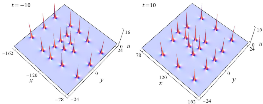
Fig. 9 Predicted solutions u_{\Lambda}(x, y, t) with \Lambda = (3, 4, 5, 7, 9) at time values of t = -10 (left) and t = 10 (right)
