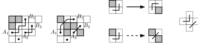
Fig. 2. Paths corresponding to two generalized excited diagrams, the flips of paths in type I and II excited moves, and the forbidden path configuration.
