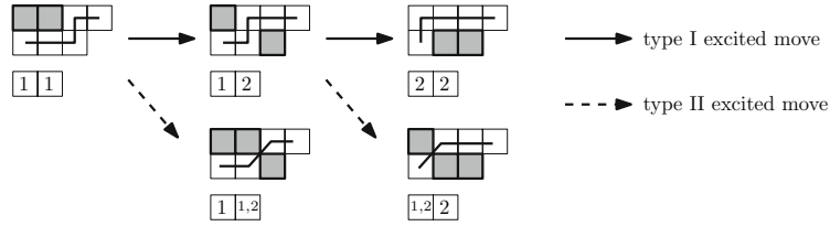
Fig. 3. The generalized excited diagrams of shape \lambda/\mu = 43/2 , their peaks, and the corresponding flagged set tableaux (see Sec. 7.5). The complements of diagrams in \mathcal{D}(\lambda/\mu) can be viewed as Delannoy paths inside \lambda .
