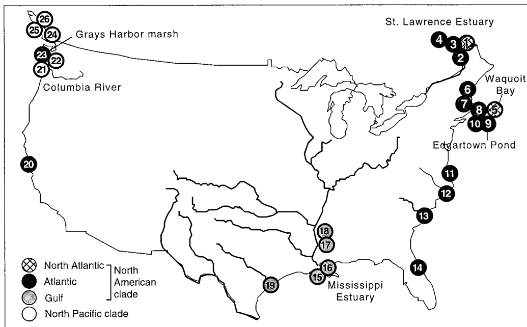
FIG. 3. Geographic distribution of three North American subclades and the North Pacific clade within the North American continent. The North Atlantic, Atlantic, and Gulf subclades belong to the North American clade, whereas the North Pacific clade is highly divergent from all the other clades (Fig. 2). Zones of contact between genetically divergent clades and subclades are in the Pacific Northwest and Atlantic Northeast regions of the North American continent near the U.S.-Canadian border.
