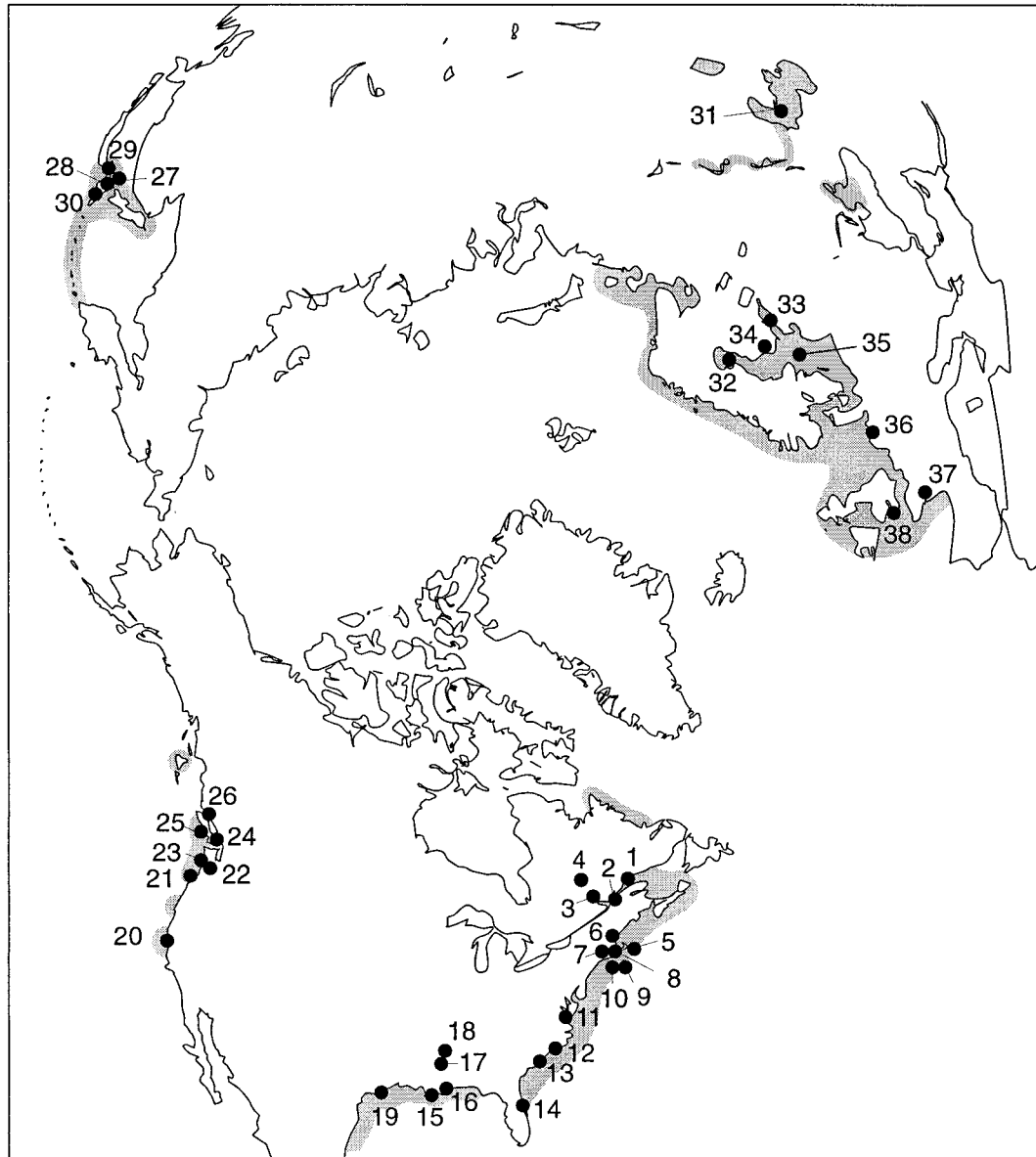
FIG. 1. Populations of Eurytemora affinis sampled for this study (represented by black dots on map with place names listed below). Gray shading shows the known distribution of E. affinis . Populations of E. affinis in northern Russia may be more widespread. (1) St. Lawrence estuary, Canada; (2) St. Lawrence marsh, Canada; (3) Saguenay River, PQ, Canada; (4) Lac St. Jean, PQ, Canada; (5) Waquoit Bay, MA; (6) Parker River pool, MA; (7) Neponset River pool, MA; (8) Oyster Pond, MA; (9) Edgartown Great Pond, MA; (10) Tisbury Great Pond, MA; (11) Chesapeake Bay, MD; (12) Cape Fear, NC; (13) Cooper River, SC; (14) St. John River, FL; (15) Fourleague Bay, LA; (16) Lake Pontchartrain, LA; (17) Black Bayou, MI; (18) Lake Beulah, MI; (19) Colorado Estuary, TX; (20) San Francisco Bay, CA; (21) Columbia River estuary, OR; (22) Chehalis River estuary, WA; (23) Grays Harbor Marsh, WA; (24) Nitinat Lake, BC, Canada; (25) Nanaimo River, BC, Canada; (26) Campbell River, BC, Canada; (27) Ishikari River, Japan; (28) Lake Baratoka, Japan; (29) Lake Ohnuma, Japan; (30) Lake Akanko, Japan; (31) Caspian Sea; (32) Gulf of Bothnia; (33) Gulf of Finland; (34) Sällvik Fjord, Finland; (35) Baltic Sea Proper; (36) IJsselmeer, Netherlands; (37) Gironde estuary, France; (38) Tamar estuary, England.
