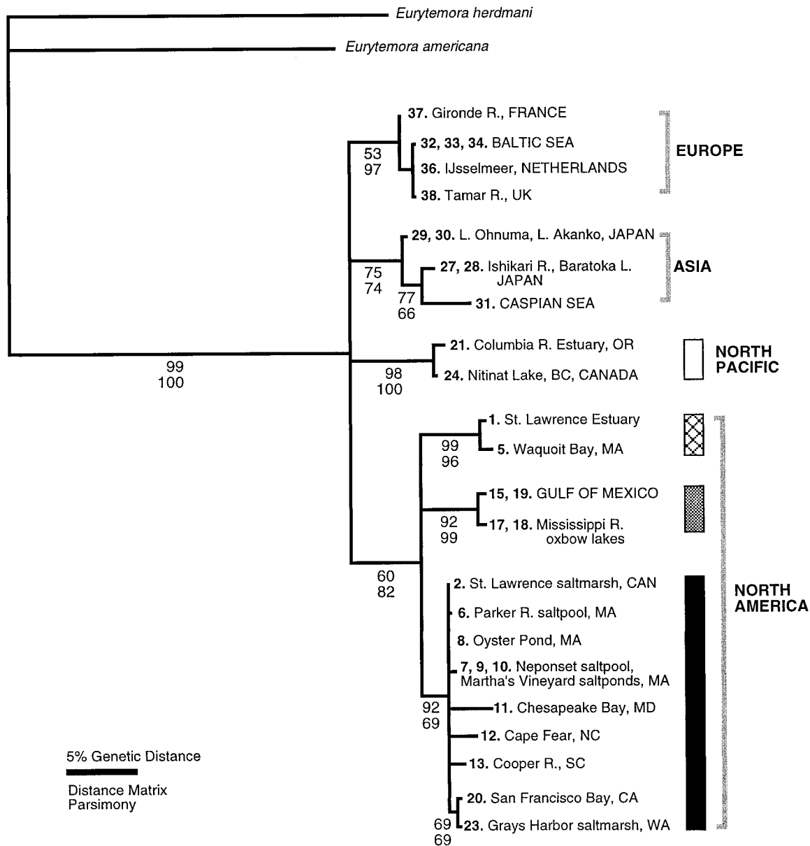
FIG. 2. Phylogeny of populations and sibling species of Eurytemora affinis using (a) 16S rRNA (450 base pairs) and (b) cytochrome oxidase I (COI, 652 base pairs). Locations of populations are shown at branch tips, with numbers designating populations as in Figure 1. Gray brackets indicate the four major clades, and thick patterned bars (a) and thick circles (b) represent distinct clades and subclades within the North American continent (see Fig. 3 for key). The trees shown were constructed with a distance matrix approach using PAUP* 4.0. Branch lengths reflect genetic distances, with scale bar indicating 5% genetic distance (maximum likelihood). The maximum-likelihood distances attempt to account for saturation of substitutions. Numbers next to nodes are bootstrap values based on 100 bootstrap replicates using distance matrix (upper number) and parsimony approaches (lower number; Felsenstein 1985). Bootstrap values of ns indicate branches not supported by values greater than 50% for a given phylogenetic method. Congeners, E. americana and E. herdmani , were used as outgroup species for 16S rRNA but not for COI because level of divergence was saturated among congeners (i.e., COI tree is unrooted).
