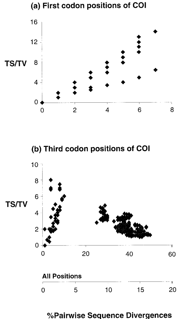
FIG. 5. Relationship between transition/transversion ratio (TS/TV) and percent pairwise sequence divergence for populations of Eurytemora affinis . (a) First codon position of COI, (b) third codon position of COI. Scale bar beneath the graphs represents the equivalent percent pairwise sequence divergence for all codon positions.
