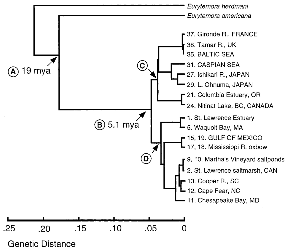
FIG. 6. UPGMA dendrogram for populations of Eurytemora affinis based on 16S rRNA gene sequences. The scale bar for genetic distance is based on a Kimura two-parameter model of evolution. Letters enclosed in circles represent major speciation events. B indicates a speciation event among major clades of E. affinis , when the polytomy in Figure 2a was formed.
