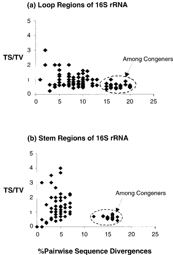
FIG. 4. Relationship between transition/transversion ratio (TS/TV) and percent pairwise sequence divergence for populations of Eurytemora affinis and congeners E. americana and E. herdmani . (a) Loop regions of 16S rRNA; (b) stem regions of 16S rRNA.
