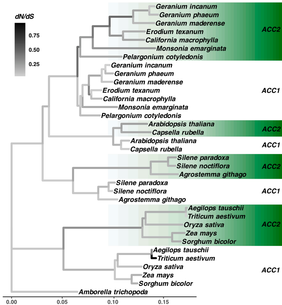
Fig. 2. ACC genes across the Brassicaceae, Caryophyllaceae, Geraniaceae, and Poaceae, with the single copy of ACC in Amborella trichopoda as an outgroup. Branch lengths represent d_N values and branch colors represent d_N/d_S ratios.
