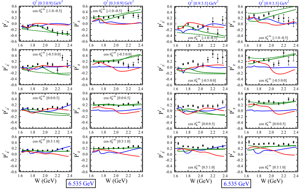
FIG. 17. Transferred \Lambda polarization components P'_{z'} and P'_z vs. W for a beam energy of 6.535 GeV. See the Fig. 13 caption for a description of the model curves and the Fig. 16 caption for details on the data.
