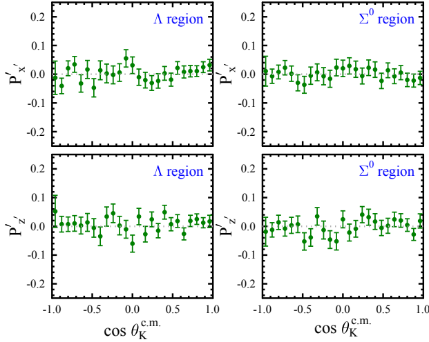
FIG. 11. Measured polarizations determined for the multi-pion background in the 6.535 GeV dataset that underlies the hyperon peaks in the MM(e'K^+) distributions for the 1D analysis vs. \cos \theta_K^{c.m.} summing over Q^2 and W for both the \Lambda (left) and \Sigma^0 (right) mass regions defined in Section III for the primed system. The error bars include the statistical uncertainties only.
