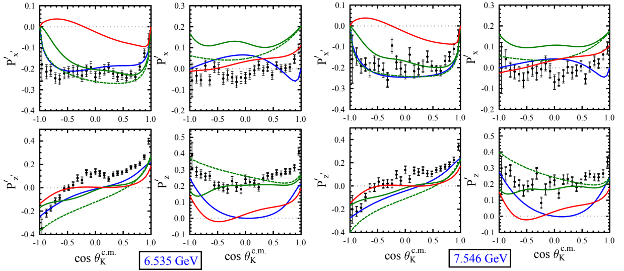
FIG. 15. Transferred \Lambda polarization components \mathcal{P}' with respect to the (x', z') and (x, z) axes vs. \cos \theta_K^{\text{c.m.}} for a beam energy of 6.535 GeV (left) and 7.546 GeV (right). See the Fig. 13 caption for details.
