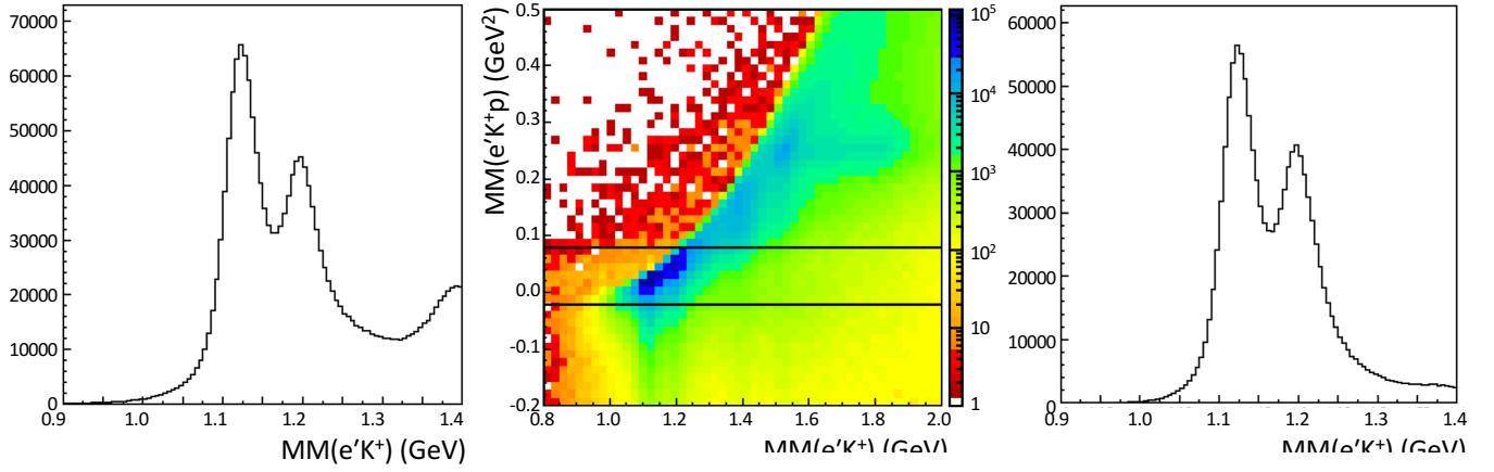
FIG. 7. (Left) MM(e'K^+) distribution requiring detection phase space showing the cut employed on the MM(e'K^+) distribution. (Right) MM(e'K^+) distribution shown in the left plot the 6.535 GeV dataset.
