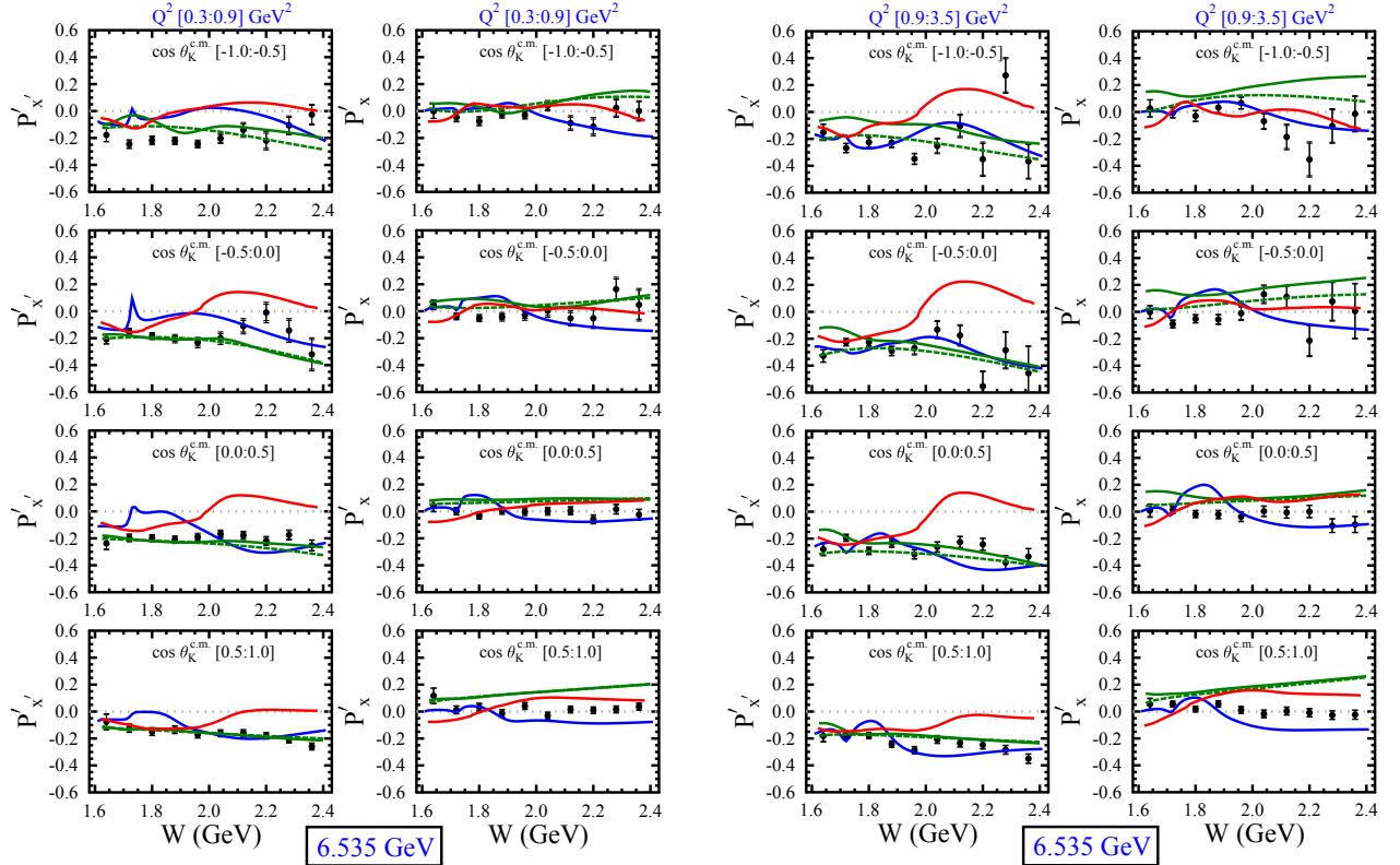
FIG. 16. Transferred \Lambda polarization components \mathcal{P}'_{x'} and \mathcal{P}'_x vs. W for a beam energy of 6.535 GeV. The data are binned in Q^2 from 0.3 to 0.9 \text{GeV}^2 (left 2x4 plots) and Q^2 from 0.9 to 3.5 \text{GeV}^2 (right 2x4 plots) for four different bins in \cos \theta_K^{\text{c.m.}} . In the text this is referred to as the 3D sort. The inner error bars on the data points represent the statistical uncertainties and the outer error bars represent the total uncertainties. See the Fig. 13 caption for a description of the model curves.
