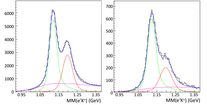
FIG. 8. Representative MM(e'K^+) fit results using hyperon templates derived from Monte Carlo ( \Lambda : green curve, \Sigma^0 : red curve) and a background template based on beam data (magenta curve). The blue curve shows the full fit result. The fits shown are from the 1D analysis binned in Q^2 with the left plot for Q^2 from 0.6-0.7 GeV 2 and the right plot for Q^2 from 2.8-3.1 GeV 2 from the 6.535 GeV dataset.
