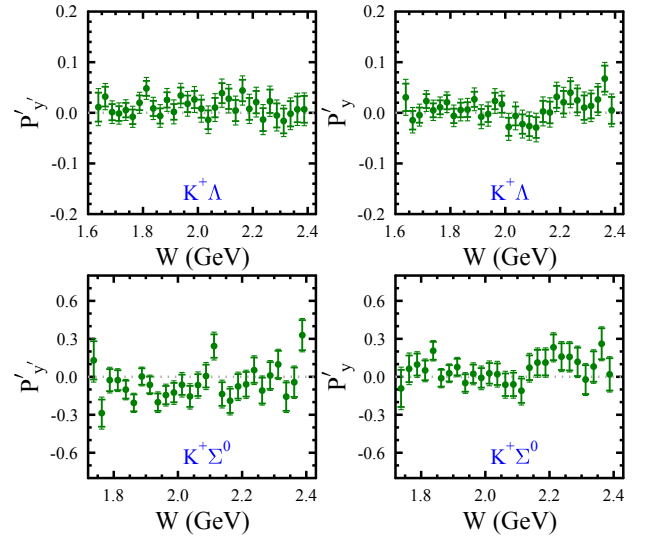
FIG. 12. Distributions of the transferred \Lambda (top) and \Sigma^0 (bottom) polarization components in relative to the y' -axis (left) and y -axis (right) vs. W from the 1D data analysis. The data shown are from the higher statistics 6.535 GeV dataset. The inner error bars on each data point represent the statistical uncertainties and the outer error bars represent the total uncertainties.
