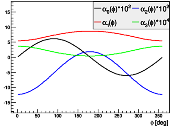
FIG. 4. Coefficients presented in Eqs. (7) to (10). Note the prescaling factors used for \alpha_0 , \alpha_2 , and \alpha_3 .
