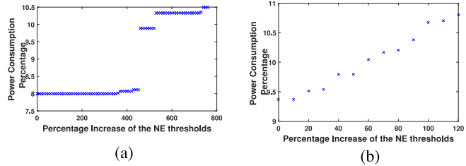
Fig. 3. Satisfaction equilibria that lead to strictly greater energy efficiency score with lower power consumption.
