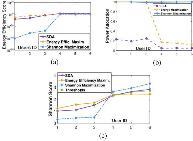
Fig. 5. Comparison of strategies for SDA, energy efficiency maximization, and Shannon maximization.
