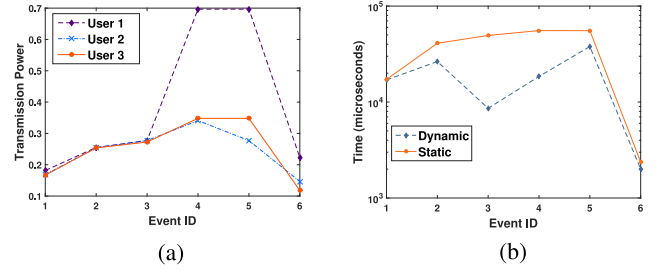
Fig. 4. SDA static and dynamic operation.
