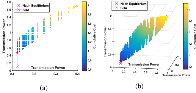
Fig. 2. Satisfaction equilibria and convergence of the SDA algorithm in a two- and three-user power control game.
