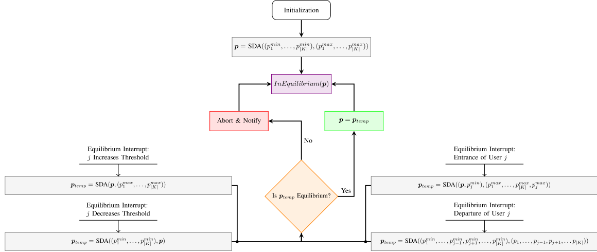
Fig. 1. Flow diagram of the holistic framework
