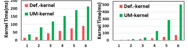
Figure 2: Hidden latency during kernel launch under Def. and UM models. (a) MatAdd . (b) MatMul .
