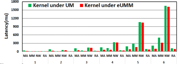
Figure 6: Kernel execution time under UM and eUMM models on TX2. The data sizes are chosen as the same sizes in Figure 5.
