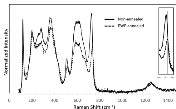
Figure 2: Effect of annealing on \text{Ti}_3\text{C}_2\text{T}_x Raman peaks. The inset figure shows the most significant Raman shift that happens at 726.5 cm -1 .
