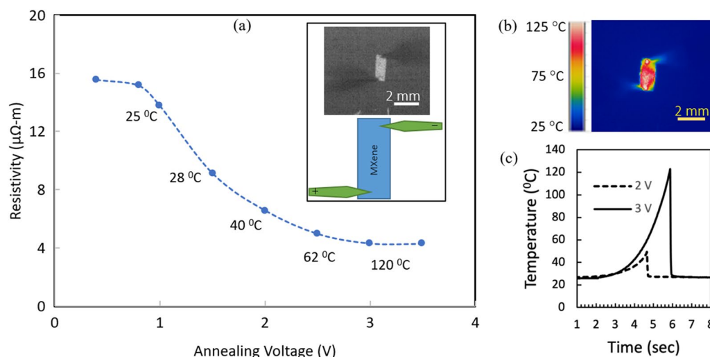
Figure 1: Effect of annealing voltage during EWF application on the resistivity of the \text{Ti}_3\text{C}_2\text{T}_x MXene films and their temperature. (a) Voltage vs. resistivity curve. We sourced the voltage and measured the current to find resistance. Inset shows the digital photo (top) and schematic (bottom) of the measurement setup. (b) IR image of MXene at 3 V. (c) Time-temperature graph of the MXene film at 2 and 3 V.
