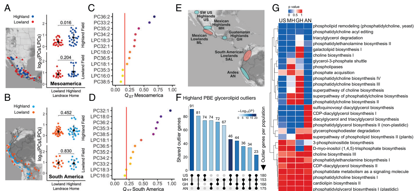
Fig. 1. Phospholipid selection in highland maize. (A and B) Left: Geographical origin of 120 maize accessions from the HiLo diversity panel used in the common garden experiment for glycerolipid quantitation. Right: PC/LPC ratio, \log_{10} scaled, for highland and lowland landraces from (A) Mesoamerica, n = 54 . The black circle indicates the mean, and the vertical line is the SD. Significant differences were tested with a false-discovery rate (FDR)-adjusted t test; the resulting P values are shown. (C and D) Q_{ST} - F_{ST} analysis of phospholipids between highland and lowland landraces from (C) Mesoamerica and (D) South America. Red line, neutral F_{ST} + 2 SD. (E–G) Highland vs. lowland PBE analysis. (E) PBE geographical sampling. (F) PBE outlier counts for glycerolipid genes in four highland populations. Bar shade indicates Fisher's exact significance test for excess shared outliers. (G) Highland selection of glycerolipid-related pathways using PBE. The heatmap shows the probability of randomly sampling gene SNPs with mean PBE greater than the mean for the gene SNPs in each pathway.
