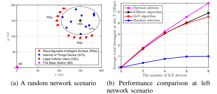
Fig. 12. (a) A random network scenario in a 200 \text{ m} \times 200 \text{ m} square area with K = 10 . (b) The performance of the optimal solution, the E2Boost algorithm, the original GoT algorithm, and the random selection method versus the number of IoT devices at 10^3 random network scenarios of the left figure.
