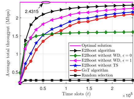
Fig. 8. The performance of different algorithms versus time slot with optimal phase shift setting when \nu_1 = \nu_2 = 2,000 , Z = 10 in a fixed network scenario of Fig. 4.
