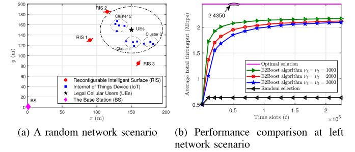
Fig. 11. (a) A random network scenario in a 200 \times 200 m square area with K = 3 , N = 11 . (b) The performance of different algorithms versus time slot with optimal phase shift setting over 10^3 random network scenarios.
