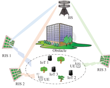
Fig. 1. A RIS-assisted hybrid uplink network.
