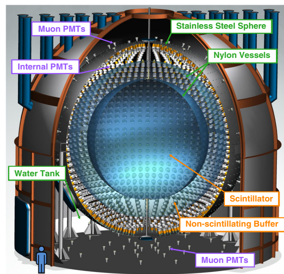
FIG. 1. Schematic representation of the Borexino detector.
