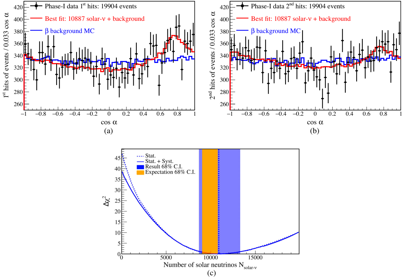
FIG. 14. The \cos \alpha distributions of the first (a) and second (b) hits of all the selected events (black points) compared with the best fit curve (red) for the resulting number of solar neutrinos N_{\text{solar-}\nu} plus background, as reported in Sec. X. All histograms are normalized to the data statistics. It can be seen that the data points cannot be explained by the background-only hypothesis (blue). (c) \Delta\chi^2 profiles of the first and second hits from the fit as a function of N_{\text{solar-}\nu} with (blue solid curve) and without (blue dotted curve) the systematic uncertainty. The no-neutrino signal hypothesis (pure background, N_{\text{solar-}\nu} = 0 ) can be rejected with \Delta\chi^2 > 25 , > 5\sigma . The 68% CI from the \Delta\chi^2 profile gives N_{\text{solar-}\nu} = 10887^{+2386}_{-2103}(\text{stat}) \pm 947(\text{syst}) , with a \chi^2/\text{ndf} = 124.6/117 . This is represented by the blue shaded band and the best fit value is shown as a vertical blue dotted line. The 68% CI of the solar neutrino signal expected based on the standard solar model (SSM) predictions [29] is shown as an orange band.
