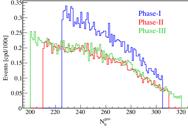
FIG. 4. The energy distributions of the data events passing the selection cuts described in Sec. V in phase I (blue), phase II (red), and phase III (green).
