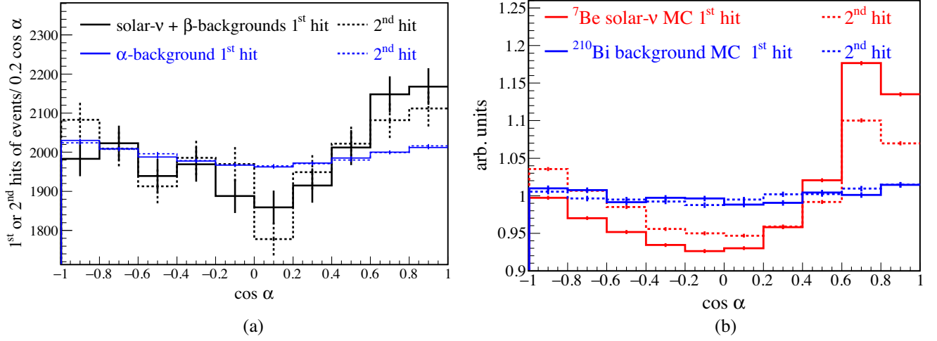
FIG. 8. Distributions of the \cos \alpha directional angle. The first hits are shown as solid lines and the second hits are shown as dotted lines. (a) \cos \alpha distribution of data events from Borexino phase I, i.e., 19904 \beta -events consisting of solar neutrinos + \beta -backgrounds (black) chosen using the selection cuts as in Sec. V and 1.8 million ^{210}\text{Po} ( \alpha ) background events (blue) in phase I. The histograms are normalized to have 19904 entries. A clear peak at positive \cos \alpha values can be observed only for the solar neutrino-rich sample. (b) \cos \alpha distributions for MC events of ^7\text{Be} solar neutrinos (red) and ^{210}\text{Bi} background (blue). The histograms are normalized to have the same area. The first hit (solid line) of ^7\text{Be} MC carries more directional information than the second hit (dotted line).
