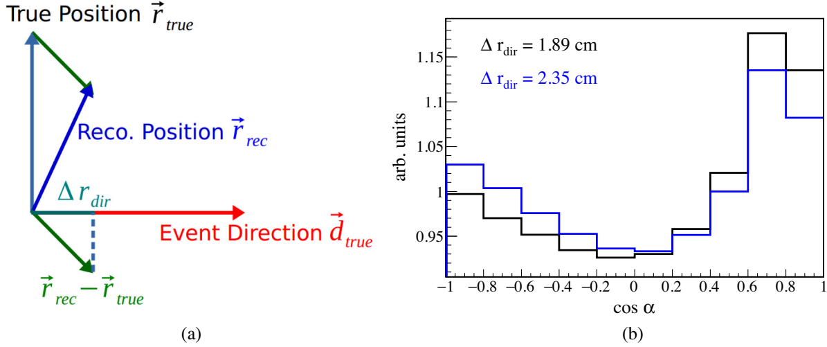
FIG. 9. (a) Effect of the biased position reconstruction \Delta r_{\text{dir}} observed in MC where the e^- position is reconstructed slightly toward the direction of the e^- . This bias of \sim 2 cm is not visible on an event-by-event basis due to the position reconstruction resolution of 12 in the ROI. (b) The effect of this parameter, where the normal {}^7\text{Be} MC has \Delta r_{\text{dir}} = 1.89 cm (black). For comparison, a larger \Delta r_{\text{dir}} = 2.35 cm (blue) increases the slope at \cos \alpha = -1 .
