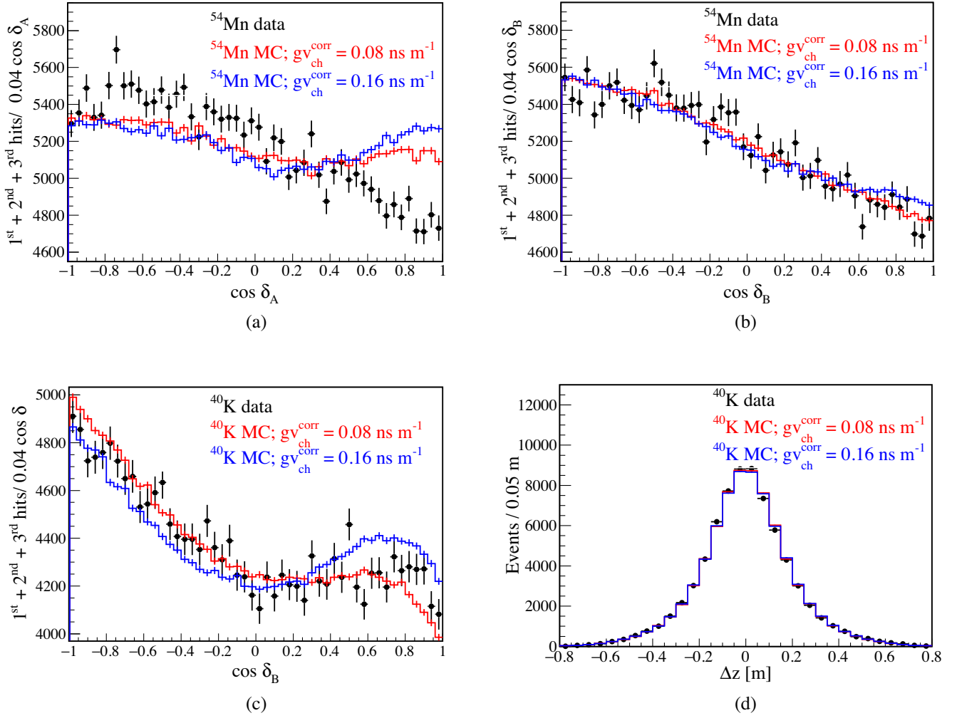
FIG. 12. Example of the effect of using separate, modified direction reconstruction PDFs, for data and MC \gamma sources for two different values of gv_{\text{ch}}^{\text{corr}} : 0.08 \text{ ns m}^{-1} (red), 0.16 \text{ ns m}^{-1} (blue). (a) \cos \delta distributions of the ^{54}\text{Mn} source where the direction of data (black) and MC (red, blue) are reconstructed with the same unmodified direction reconstruction PDF. (b) \cos \delta distributions of the same ^{54}\text{Mn} source for one scenario where the direction is reconstructed with different, modified PDFs for data and both gv_{\text{ch}}^{\text{corr}} MC simulations. The PDFs are selected to give a good agreement for the \cos \delta distributions. (c) \cos \delta distributions of the ^{40}\text{K} source with the same combination of direction reconstruction PDFs that are used for ^{54}\text{Mn} in (b). (d) Position reconstruction of data (black) and MC (red, blue) with the modified position reconstruction PDFs that are also used for (b), (c). Both the modification of the PDFs and the Cherenkov group velocity correction gv_{\text{ch}}^{\text{corr}} do not impact the position reconstruction performance, as shown for ^{40}\text{K} .
