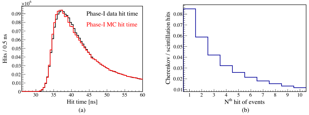
FIG. 7. (a) Time-of-flight corrected hit times for phase I data (black) and MC (red) in the ROI, where the MC is normalized to data statistics. Both ^7\text{Be} and ^{210}\text{Bi} MC are comparable within their statistics and only ^7\text{Be} is shown. (b) Ratio of detected Cherenkov-to-scintillation hits as a function of the time-of-flight sorted hits for all events of ^7\text{Be} MC.
