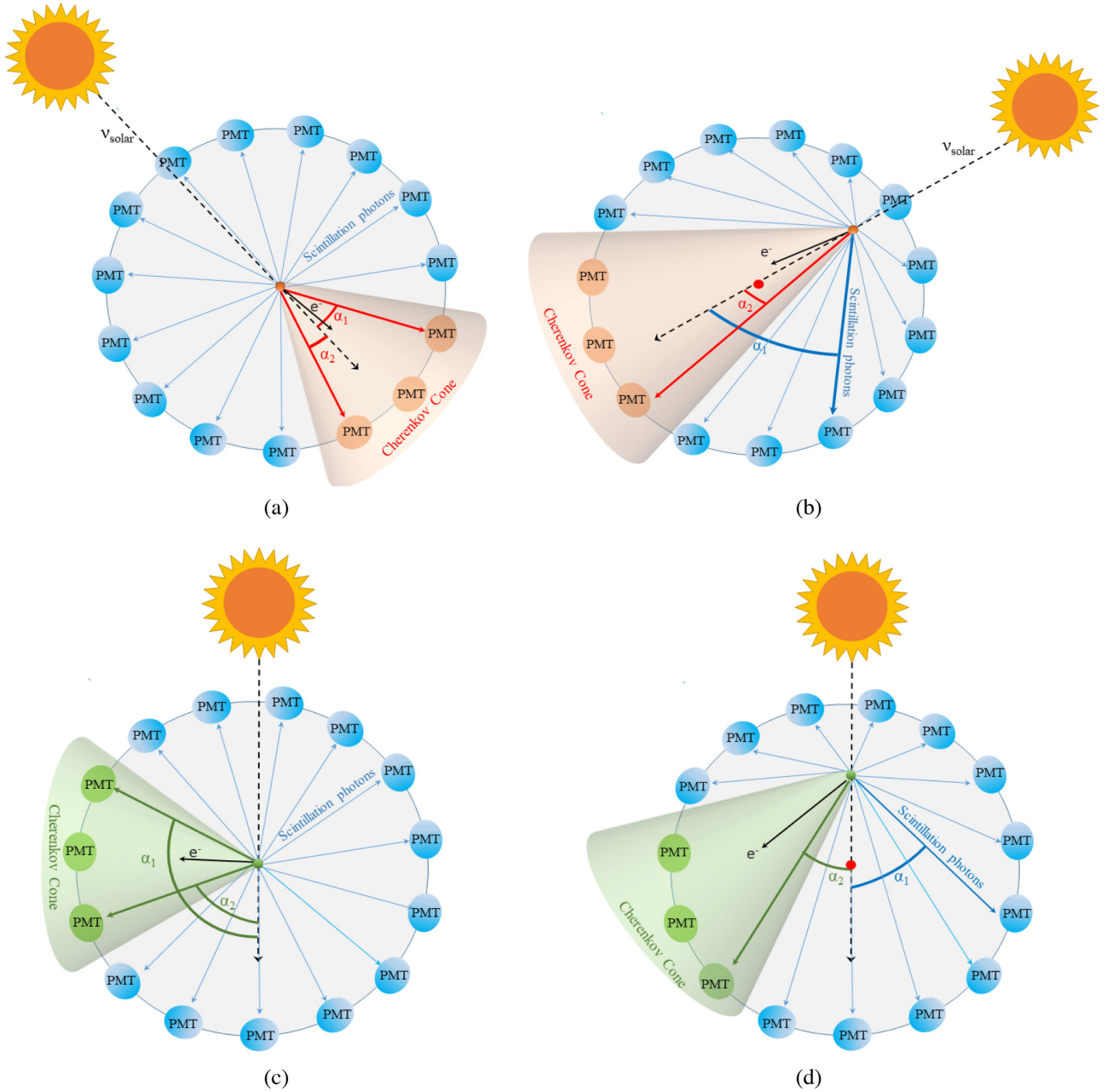
FIG. 3. Schematic representation of the angular correlation, expressed by the angle \alpha between the direction of emitted photons, given by the reconstructed vertex, and the position of the Sun with respect to Borexino for different event types. (a) Electron recoiling off a solar neutrino at the center of the detector produces a Cherenkov cone (red arrows) pointing forward in the direction of the Sun and isotropic scintillation photons (blue arrows). \alpha_1 and \alpha_2 are the directional angles of the first and second detected photons of the event, respectively. The Cherenkov photons and, in turn, the PMT hits they trigger are correlated to the incoming direction of the solar neutrinos. (b) It is possible that the first detected photon in an event is a scintillation photon, therefore not correlated to the direction of the solar neutrino, and the second detected photon is a Cherenkov photon. Compared to (a), this event results in a flatter angular distribution. In addition, this event happens off-center. (c) An electron from the intrinsic radioactive background also produces a Cherenkov light cone (green arrows) and isotropic scintillation photons (blue arrows). As before, \alpha_1 and \alpha_2 are the directional angles of the first and second photons of the background event, respectively. These are Cherenkov photons, but have no correlation to the Sun's direction. (d) Background event similar to (c), but this is an off-center event where the first photon is a scintillation photon and the second detected photon is a Cherenkov photon.
