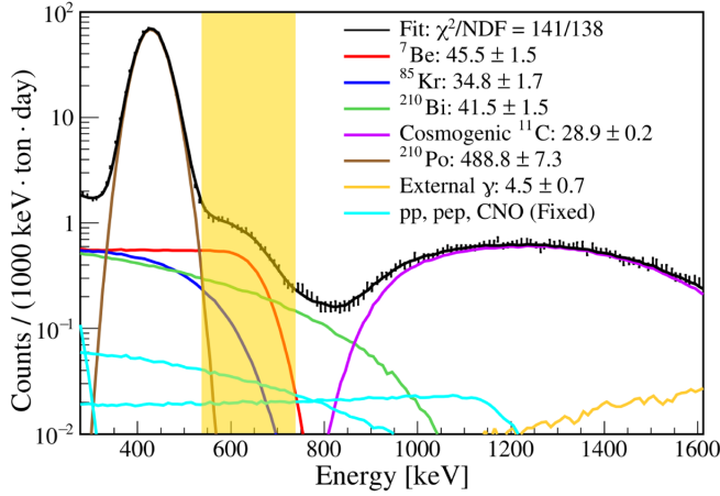
FIG. 2. The spectral fit of the energy spectrum performed in phase I [20]. The PDFs of the different solar neutrino components and backgrounds are also shown along with the fitted data. The energy region of interest (ROI) used for the directional analysis of phase I is shown as a shaded yellow area.
