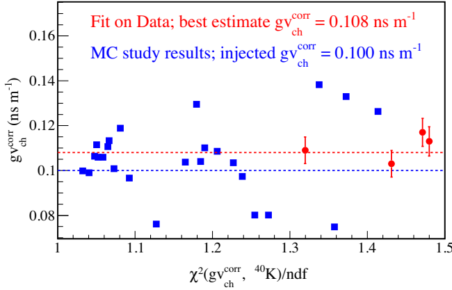
FIG. 13. The g v_{\text{ch}}^{\text{corr}} fit results of the gamma Cherenkov calibration as a function of \chi^2/\text{ndf} of the ^{40}\text{K} \cos \delta histograms [Eq. (8)]. The red data points are the g v_{\text{ch}}^{\text{corr}} estimated from the fit between data and MC, for which the best estimate 0.108 \text{ ns m}^{-1} is given by the red dotted line. The blue squares represent the extracted g v_{\text{ch}}^{\text{corr}} from MC studies, falling in the same \chi^2/\text{ndf} space, for an injected g v_{\text{ch}}^{\text{corr}} = 0.10 \text{ ns m}^{-1} represented by the blue dotted line.
