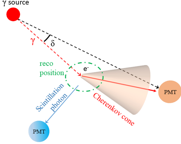
FIG. 10. Schematic representation of the \cos \delta angle used for the Cherenkov calibration with gamma sources. A \gamma (red dashed line) is emitted from the calibration source position \vec{r}_{\text{source}} (red filled circle). The Compton-scattered e^- s (red solid line) in turn emit Cherenkov light (orange cone) in correlation to the direction of the incident \gamma . The direction of scintillation photons (blue) are uncorrelated to the \gamma direction. The directional angle \delta used for the calibration of the Cherenkov light in this analysis is the angle between the reconstructed gamma direction (based on the reconstructed position \vec{r}_{\text{rec}} (green circle)) and the photon direction of the hit (based on the known source position and the PMT position \vec{r}_{\text{PMT}} ), as defined in Eq. (5).
