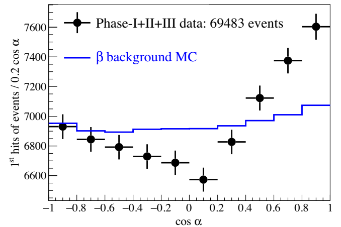
FIG. 15. The \cos \alpha distribution of phase I + phase II + phase III data events, compared with the \beta background MC PDF normalized to the statistics of data. It can be seen that the data cannot be explained with a background-only hypothesis.
