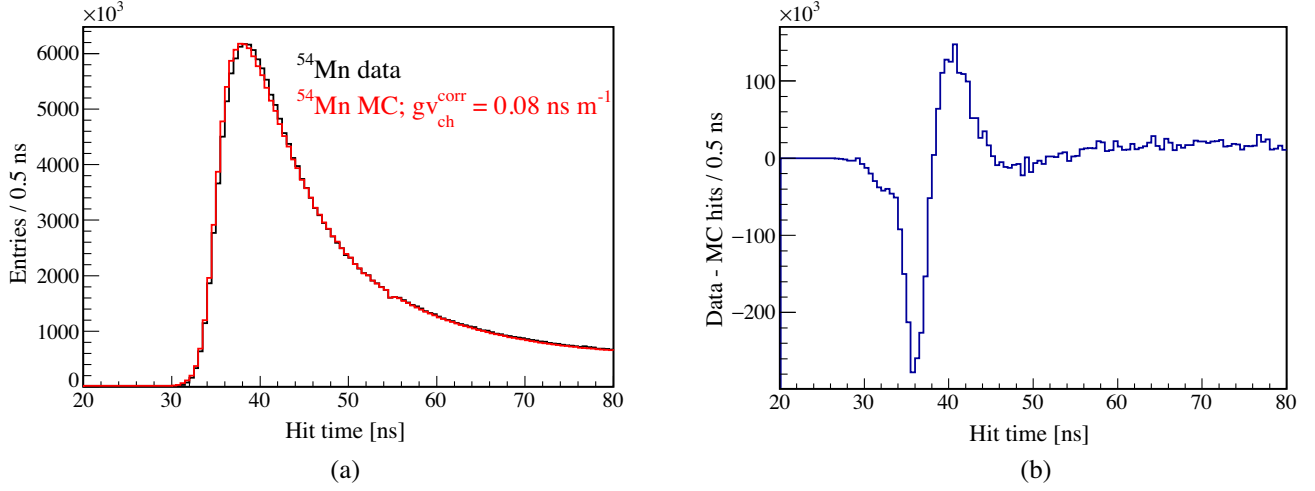
FIG. 11. (a) Time-of-flight corrected hit times for PMT hits of all events in data (black) and MC (red) of the ^{54}\text{Mn} gamma calibration source. The distributions are normalized to have the same area. (b) The difference between the data and MC time distributions in (a).
