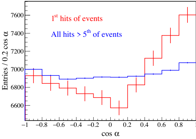
FIG. 5. The \cos \alpha distribution of the selected data events for phase I + II + III. The very first hit (red) of all the events after time-of-flight correction is compared to all the hits detected later than the > 5^{\text{th}} time ordered hit of the events (blue). The histograms are normalized to the same statistics.
