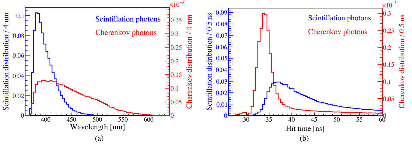
FIG. 6. (a) Borexino Monte-Carlo wavelength spectra as detected by the PMTs. (b) Monte-Carlo distributions of the hit times corrected with their time-of-flight for {}^7\text{Be} solar neutrino recoil electrons (0.54 MeV to 0.74 MeV). In both figures, the left y-axis shows the scintillation (blue), where the area is normalized to 1 and the right y-axis corresponds to Cherenkov light (red), normalized to the number of Cherenkov hits relative to scintillation ( \sim 0.4\% ). Both scintillation profiles also include those photons that have been produced in the Cherenkov process, but have been absorbed and reemitted by the LS.
