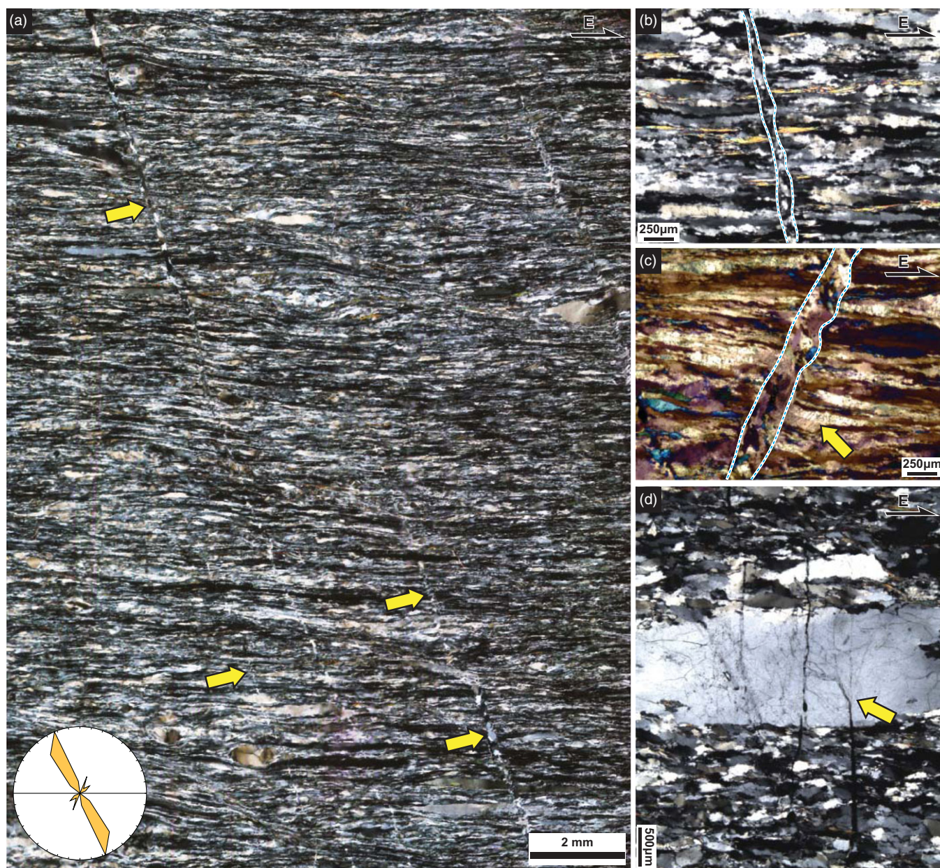
Fig. 4. (Colour online) Cross-polarized photomicrographs of thin-sections oriented perpendicular to the foliation and parallel to the lineation. (a–c) Microcracks tend to be oriented at a high angle to the mylonitic foliation (see circular frequency polygon). They are filled with quartz, which has a distinct fabric, not as strong as the mylonitic fabric, suggesting that microcracks healed while the shear zone was still at conditions favourable for quartz crystal plasticity. Fluid inclusions are abundant within the quartz fill and seem to be forming fluid inclusion planes that are sub-parallel with the walls of the microcracks (yellow arrow). (d) Horsetail structures (yellow arrow) are commonly found at the tip of mineralized microcracks. These structures contain a large number of fluid inclusion planes that typically fan out both upward and downward at the tip of the cracks.
