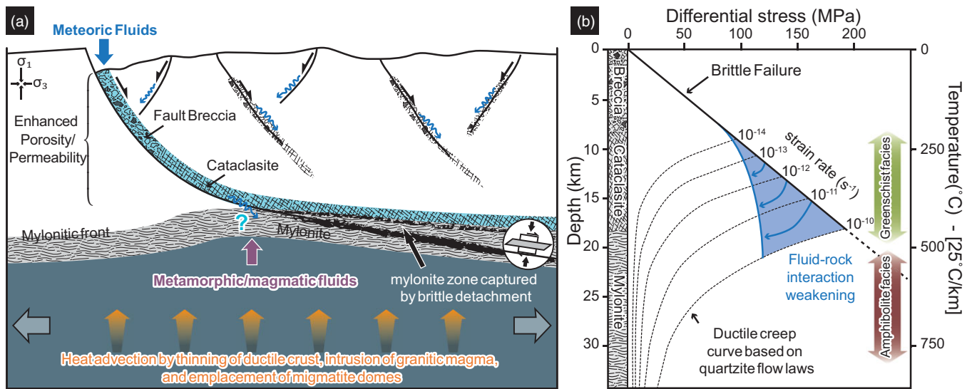
Fig. 1. (Colour online) (a) Fluid–rock interaction in a detachment system associated with the formation of a metamorphic core complex and (b) strength profile through the crust plotted with Coulomb frictional failure criterion for the upper crust and quartzite flow law for the lower crust, using a 25 °C/km geothermal gradient (modified from Gottardi et al. 2018).
