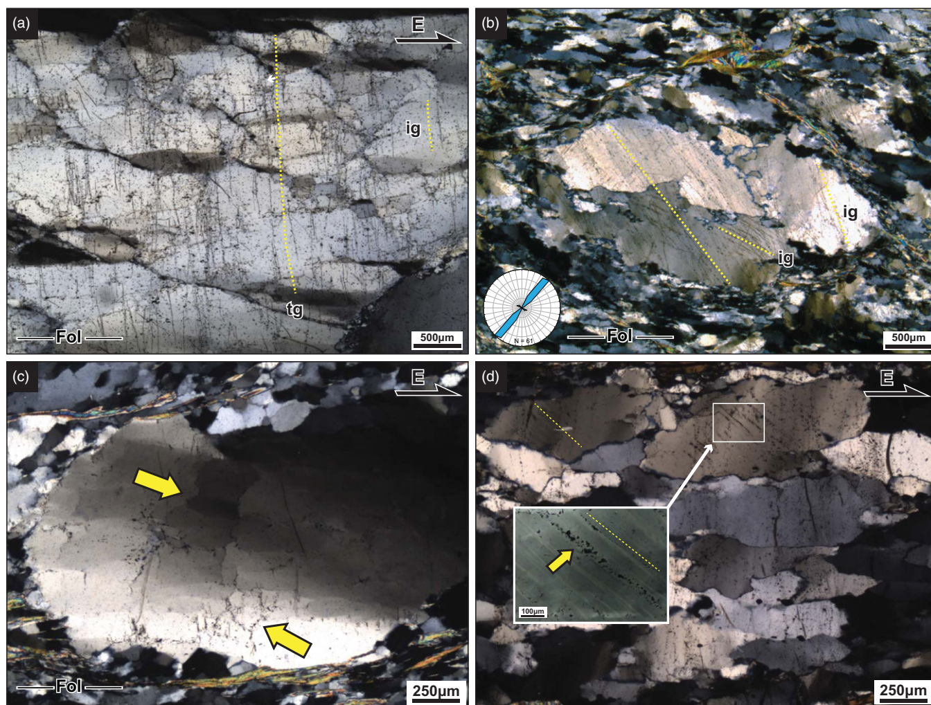
Fig. 6. (Colour online) Cross-polarized photomicrographs of thin-sections oriented perpendicular to the foliation and parallel to the lineation. Fluid inclusion planes cross multiple grains (transgranular, tg) and single grains and subgrain boundaries (intergranular, ig). (a) In boudinaged vein samples collected near the top of the detachment shear zone, transgranular fluid inclusion planes are oriented sub-perpendicular to the mylonitic foliation (Fol). (b) In quartzite mylonite samples collected at deeper structural levels, the transgranular fluid inclusion planes occur in two conjugate orientations, dipping at \sim 40\text{--}60^\circ from the mylonitic foliation. These transgranular fluid inclusion planes typically cut across elongate relict quartz grains that define the mylonitic foliation and can be hundreds of microns long. Individual fluid inclusion planes (FIP) typically preserve a high number of fluid inclusions. (c) Grain boundary fluid inclusions are common in the quartzite mylonite. They are either found around recrystallized quartz grains or they outline subgrain boundaries in large relict grains (yellow arrows). (d) Deformation lamellae are found in 20–50 % of quartz grains in the quartzite mylonite (dashed yellow lines). They are very well developed in large quartz grains that are elongated at a high angle to foliation but occur also in smaller recrystallized grains. Deformation lamellae are commonly decorated by fluid inclusions (yellow arrow).
