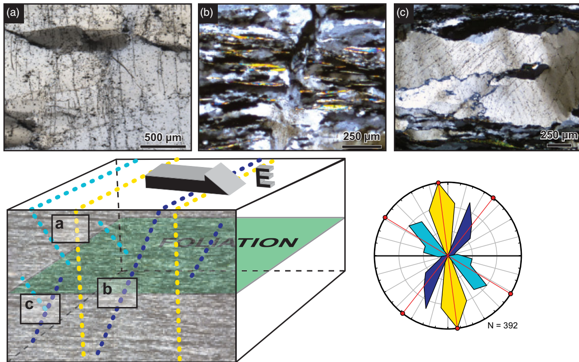
Fig. 10. (Colour online) Composite frequency polygon and block diagram representing the general orientation of brittle microstructures (healed microfractures and transgranular fluid inclusion planes) with respect to the mylonitic foliation and lineation.
