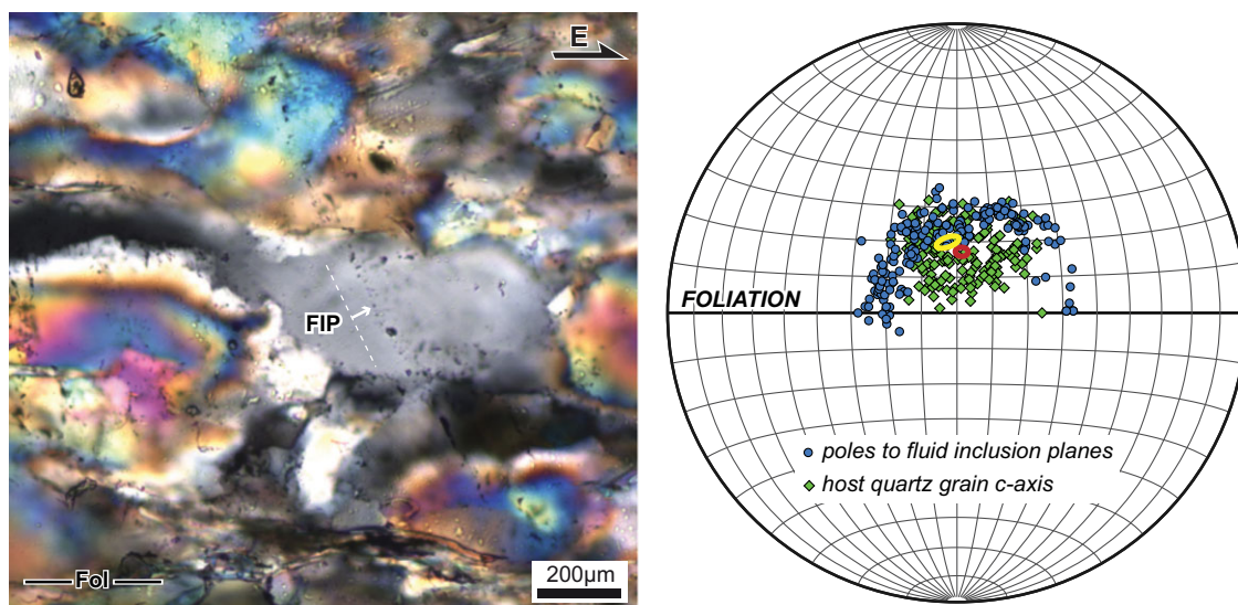
Fig. 9. (Colour online) (Left) Cross-polarized photomicrograph of the quartzite mylonite showing quartz grain (grey, in the centre of the image) with fluid inclusion plane (FIP). (Right) Equal-area, lower-hemisphere stereographic projections of the orientation of poles to planes of intragranular fluid inclusions and host quartz c-axes, measured with respect to the mylonitic foliation.
