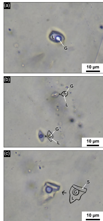
Fig. 8. (Colour online) Plain-polarized photomicrographs of thin-sections oriented perpendicular to the foliation and parallel to the lineation. (a) Inclusion with dark rims, possibly indicative of high-density fluid. (b) Photomicrograph of a two-phase fluid inclusion with large inner phase that is stationary. (c) Photomicrograph of a three-phase fluid inclusion that has stationary inner phases. L – liquid; G – gas (vapour bubble); S – solid.
