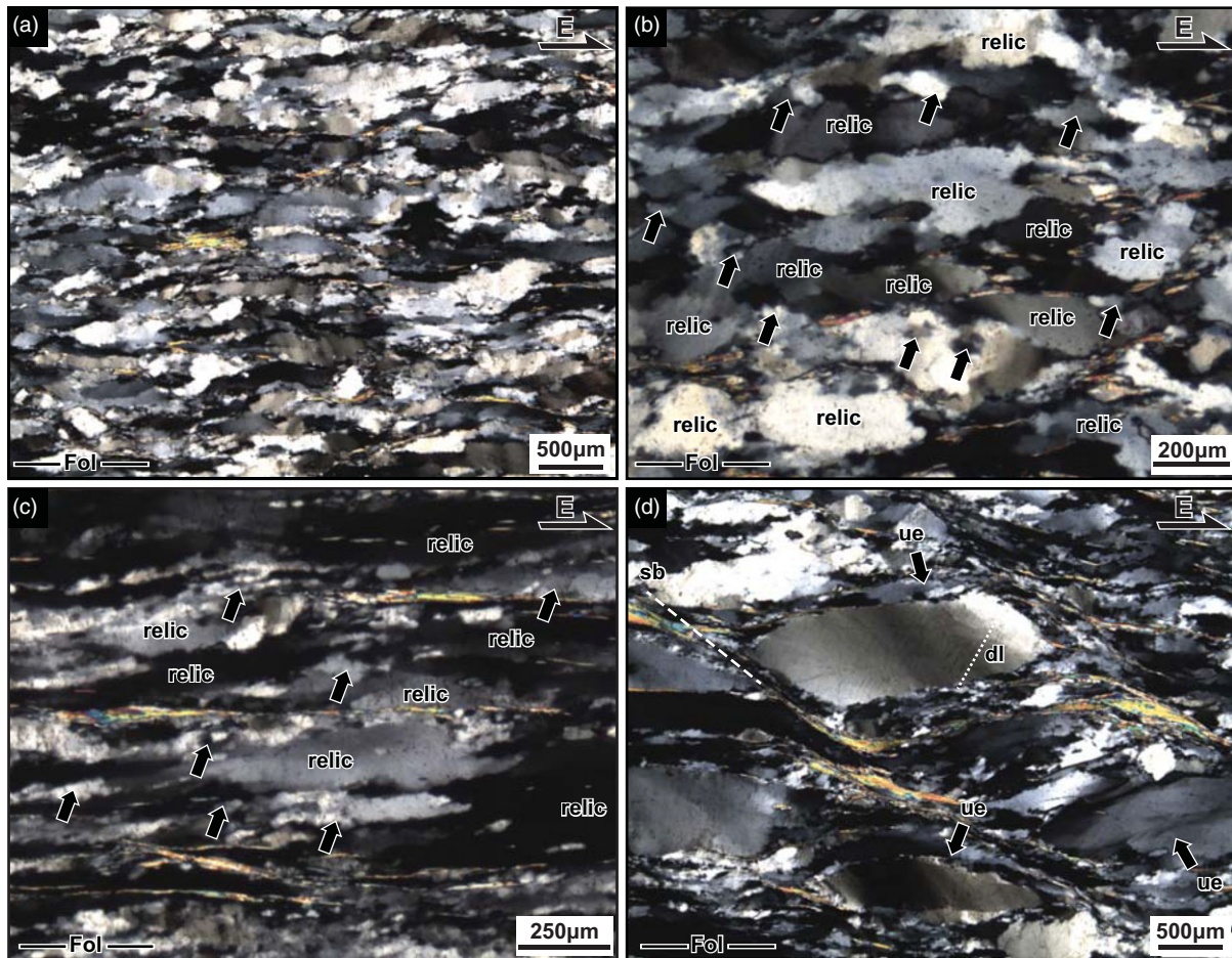
Fig. 3. (Colour online) Cross-polarized thin-section photomicrographs showing (a) representative quartz and muscovite microstructures of the Elba Quartzite mylonite from the Raft River detachment shear zone. (b, c) The quartz grain population is divided into large relict grains and small recrystallized grains (arrows). (d) Relict grains show strong undulose extinction (ue) and commonly contain deformation lamellae (dl). When present, shear bands (sb) form at a shallow angle ( \sim 10\text{--}20^\circ ) to the mylonitic foliation. Thin-sections cut perpendicular to foliation (fol) and parallel to lineation; the photomicrographs are taken oriented top-to-the-E.
