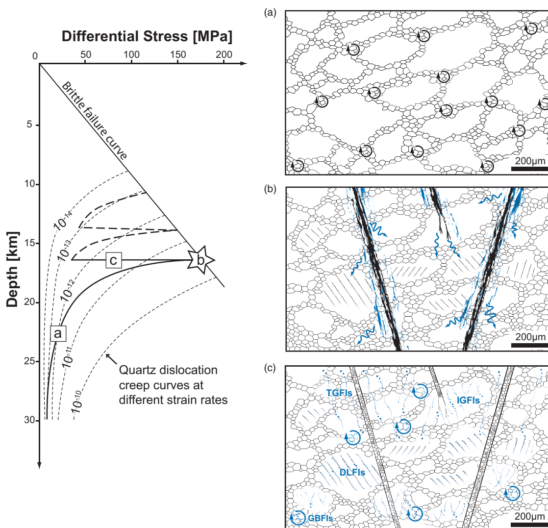
Fig. 11. (Colour online) Model for fluid circulation based on the various fluid-related microstructures observed in the Raft River detachment shear zone. Crustal strength profile of the continental crust, using Byerlee's law (Sibson, 1974) for the brittle upper crust and the Hirth et al. (2001) quartzite dislocation creep flow law for the lower crust. (a), (b), (c) show potential differential stress pathways for the observed microstructures. (a) During stress build-up, deformation of the quartz grain is accommodated by dislocation creep subgrain rotation recrystallization. (b) Strain hardening leads to embrittlement and eventually seismic brittle failure, forming faults, fractures and microcracks, which allow for surface fluids to be pumped into the shear zone. (c) Post-seismic relaxation heals fractures and traps the fluids as transgranular fluid inclusions (TGFIs) and intergranular fluid inclusions (IGFIs). Continued crystal-plastic deformation by subgrain rotation and grain boundary migration redistributes small fluid inclusions as grain/subgrain boundary fluid inclusion clusters (GBFIs).
