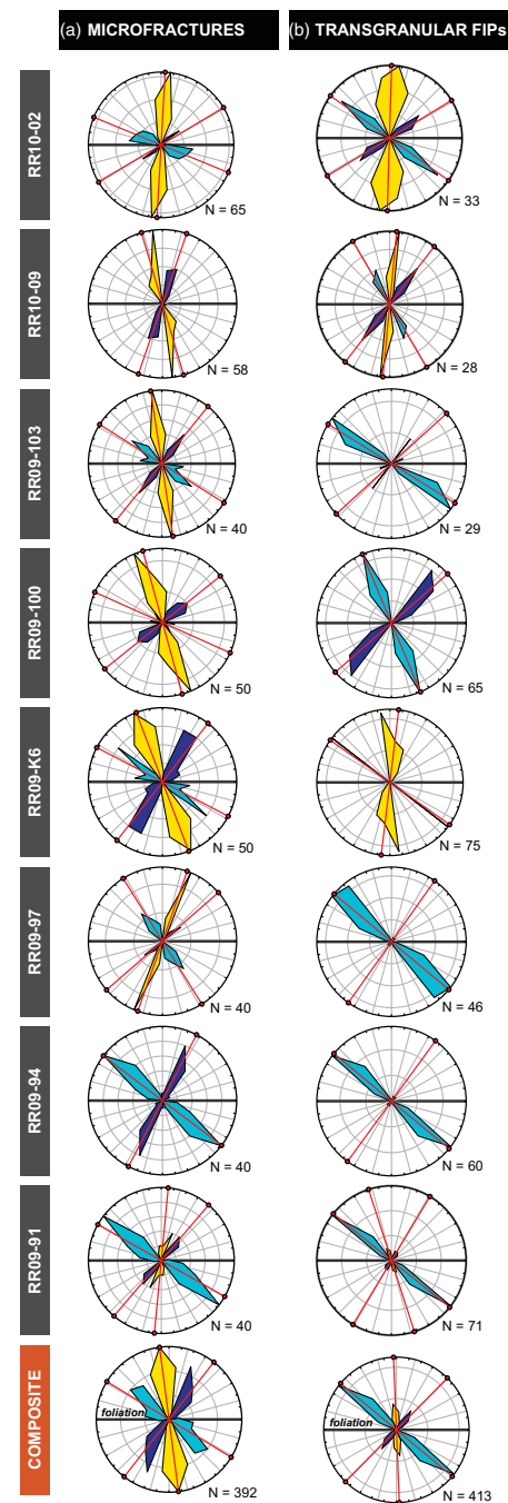
Fig. 5. (Colour online) Orientations of (a) healed microfractures and (b) transgranular fluid inclusion planes (FIPs) within both mylonite and quartz vein samples. Frequency polygons of each sample and the composite frequency polygon show three sets of healed microfractures: one set sub-perpendicular to the mylonitic foliation (yellow) and two conjugate sets. The conjugate sets are oriented \sim 30^\circ \pm 10^\circ (light blue) and \sim 130^\circ \pm 10^\circ (dark blue) for the microfractures, and \sim 40^\circ \pm 10^\circ (light blue) and \sim 135^\circ \pm 10^\circ for the transgranular fluid inclusion planes, clockwise with respect to the mylonitic foliation (central black line on the frequency polygon, labelled on the composite diagram). The red line on the frequency polygon indicates the average of the specific cluster. The block diagram represents the schematic orientation of these three sets of healed microfractures with respect to the mylonitic fabric. See Figure 2c for sample location.
