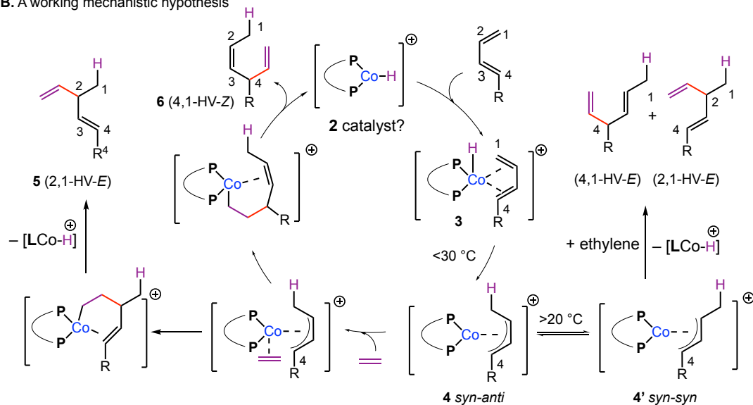
Figure 2. Co-catalyzed HV of 1,3-dienes
