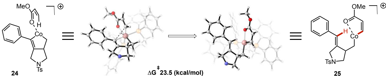
Figure 10. Cycloisomerization/regiodivergent hydroalkenylation of 1,6-enynes
