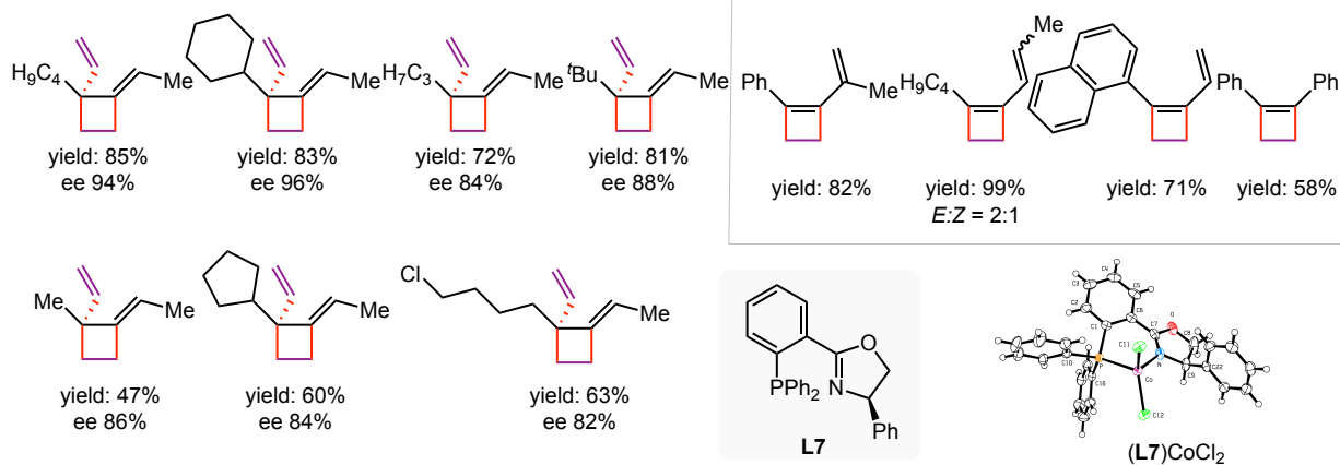
Figure 9. Cyclobutanes via tandem [2+2]-cycloaddition/hydrovinylation
