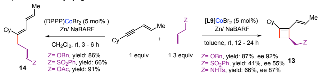
Figure 7. Enantioselective cobalt-catalyzed [2+2]-cycloadditions
