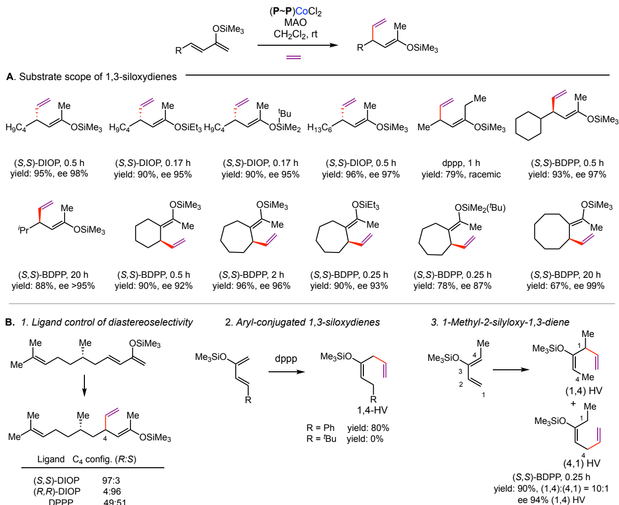
Figure 4. Enantioselective HV of siloxydienes. \beta -Vinyl silyl enol ethers
