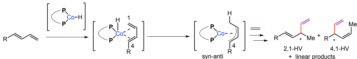
Figure 1. Nickel and cobalt-catalyzed hydrovinylation reactions
