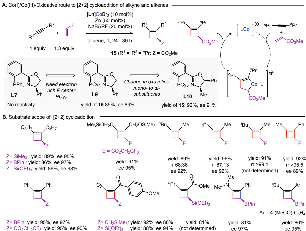
Figure 8. Fine-tuning ligands for [2+2]-cycloaddition
