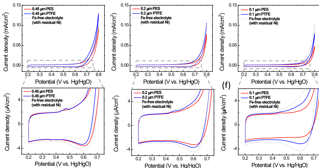
Figure 4. CV curves of Pt coil with surface area 4.1 \text{ cm}^2 at 50^{\text{th}} cycle in 10 mL of Ni-cleaned Fe-free 1 M KOH after filtering through different pore sizes (a) and (d) 0.45 \text{ }\mu\text{m} , (b) and (e) 0.2 \text{ }\mu\text{m} , (c) and (f) 0.1 \text{ }\mu\text{m} .
