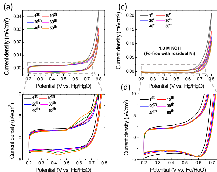
Figure 1. Cyclic voltammogram of Pt coils in \text{Ni(OH)}_2 -cleaned Fe-free (a) 0.1 M, (c) 1.0 M KOH electrolyte; (b) and (d) show the corresponding enlarged precatalytic regions with the number referring to cycle number. The electrodes show different capacitive currents because of the different-sized Pt coils used in the tests. The surface area of the Pt-coil working electrode used is 1.8 \text{ cm}^2 in 0.1 M KOH and 4.1 \text{ cm}^2 in 1.0 M KOH. The growth of a redox wave associated with \text{Ni(OH)}_2/\text{NiOOH} redox is apparent upon extended cycling in 0.1 M KOH. The apparent redox wave from \text{Ni(OH)}_2/\text{NiOOH} appears largely on the first couple cycles for the 1.0 M KOH, which suggests that the \text{Ni(OH)}_2 colloids/particulates may absorb even in the absence of bias. The precatalytic \text{Ni(OH)}_2/\text{NiOOH} features, most notably the large cathodic feature, do disappear in the further cleaned electrolyte from which Ni impurities are removed (see below) for both electrolytes.
