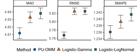
Fig. 2: Prediction performance comparison for PU-OMM, Logistic-Gamma, and Logistic-LogNormal models with the California Wildfire dataset. Average MAD, RMSE, and SMAPE values are plotted for each method. Error bars represent 1 standard error.
