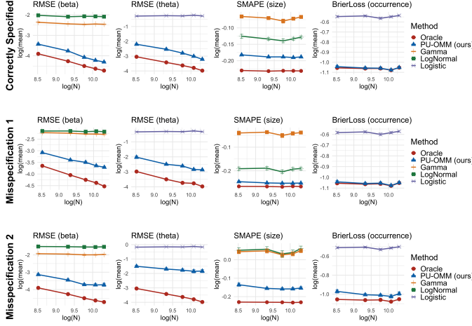
Fig. 1: Parametric estimation and prediction accuracy for each method under Settings 1-3 (Correctly Specified, Misspecification 1, and Misspecification 2). Each row i corresponds to the Setting i , for i = 1, 2, 3 . For each row, first two panels (RMSE (beta), RMSE (theta)) show parameter estimation accuracy results, and the last two panels (SMAPE (size), BrierLoss (occurrence)) plot the accuracy of each method in predicting the true size and occurrence of each observation in test datasets. Average values from B = 50 trials are plotted, together with error bars corresponding to one standard error. Note for the Logistic-Gamma and Logistic-LogNormal Mixture models, the logistic model is used to predict the occurrence of events, and Gamma/LogNormal model is used to predict the magnitudes of events. Therefore, our PU-OMM model is compared with the Gamma/LogNormal models in RMSE (beta) and SMAPE (size) panels, and PU-OMM is compared with the Logistic model in RMSE (theta) and BrierLoss (occurrence) panels.
