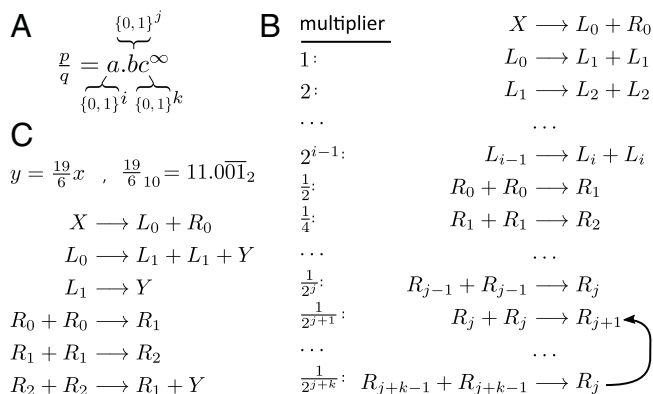
Fig. 5. Noncompetitive bimolecular rational multiplication. (A) Binary representation of rational p/q , where a, b , and c are binary strings. Strings a and b are lengths i and j , respectively, while c is an infinitely repeated string of length k . (B) A scheme for constructing a noncompetitive bimolecular CRN for rational multiplication. The reaction chain uses i + j + k + 1 reactions to “implement” the binary expansion. The last reaction creates a “loop” in the reaction chain which corresponds to string c . The number of times each reaction will be applied (before looping) is some multiple of the initial count of X , as indicated by the multiplier column. An output species Y will appear as a product for each reaction where a “1” appears in the binary expansion. (C) An example CRN which computes y = (19/6)x . Note that, to achieve a dual-rail representation, we can repeat this construction twice, for both positive ( X^+, Y^+ ) and negative ( X^-, Y^- ) input and output species.
