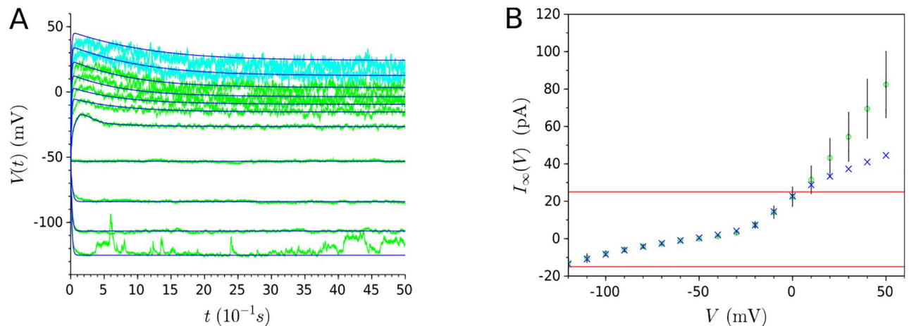
Fig 5. Results of single-objective optimization (evolution of AIY membrane potential). (A) Experimental voltages for stimuli starting from -15pA and increasing to 35pA by 5pA increments are represented in green. Estimated voltages resulting from the I_{Ca,t} + I_{Kir} + I_{K,p} + I_L -model for stimuli going from -15pA to 25pA are represented in dark blue, whereas those relative to 30pA and 35pA are represented in light blue. (B) Experimental steady-state currents (represented by green circles) and estimated steady-state currents (represented by blue crosses) resulting from the fitting of membrane potential evolution in (A). Red lines delineate the interval [-15pA; 25pA].
