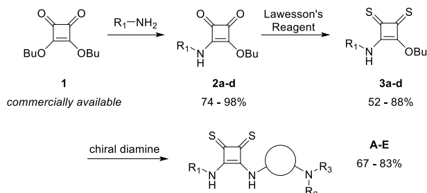
Figure 2. Synthesis of Bifunctional Thiosquaramides via the Vinylogous Butyl Ester
