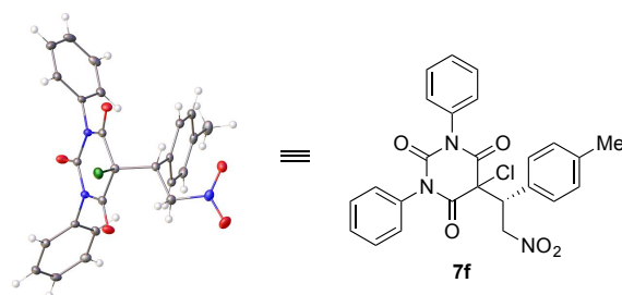
Figure 4. X-ray Crystal Structure of a Chlorinated Barbiturate
