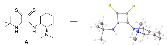
Figure 3. X-ray Crystal Structure of a Bifunctional Thiosquaramide
