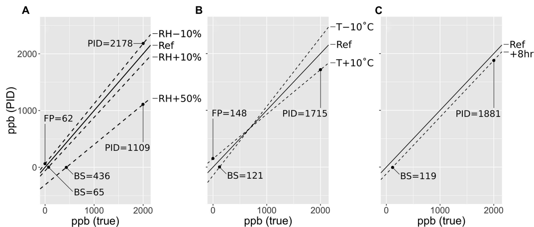
FIGURE 3 | A rough guide for assessing the importance of controlling for PID measurement error (commonly called ‘PID drift’) for a given application and environment. This figure shows estimated outcomes of PID measurements of a gas ranging from 0 to 2000 ppb using the standard onboard calibration method, and measuring under varying sample relative humidity (RH, A ), instrument temperature (T, B ), and time ( C ). Conditions are specified at the right of each panel, with ‘Ref’ representing conditions during PID calibration. Sensitivities are derived from Figure 2 . PID measurement error can manifest as ‘blind spots’ (BS) where the PID reads zero for non-zero gas concentrations, false positives (FP) where the PID reads non-zero for zero gas concentrations, and inaccuracies in non-zero gas readings (sensor responsivity). RH will be the most important concern for most users, though direct sun exposure can cause large changes in T. Controlling or correcting for PID measurement error will be most important for applications requiring lower detection limits, precision, and accuracy better than approximately 500–1000 ppb. This should be used only as a rough guide, as PID sensitivities likely differ between sensors.
