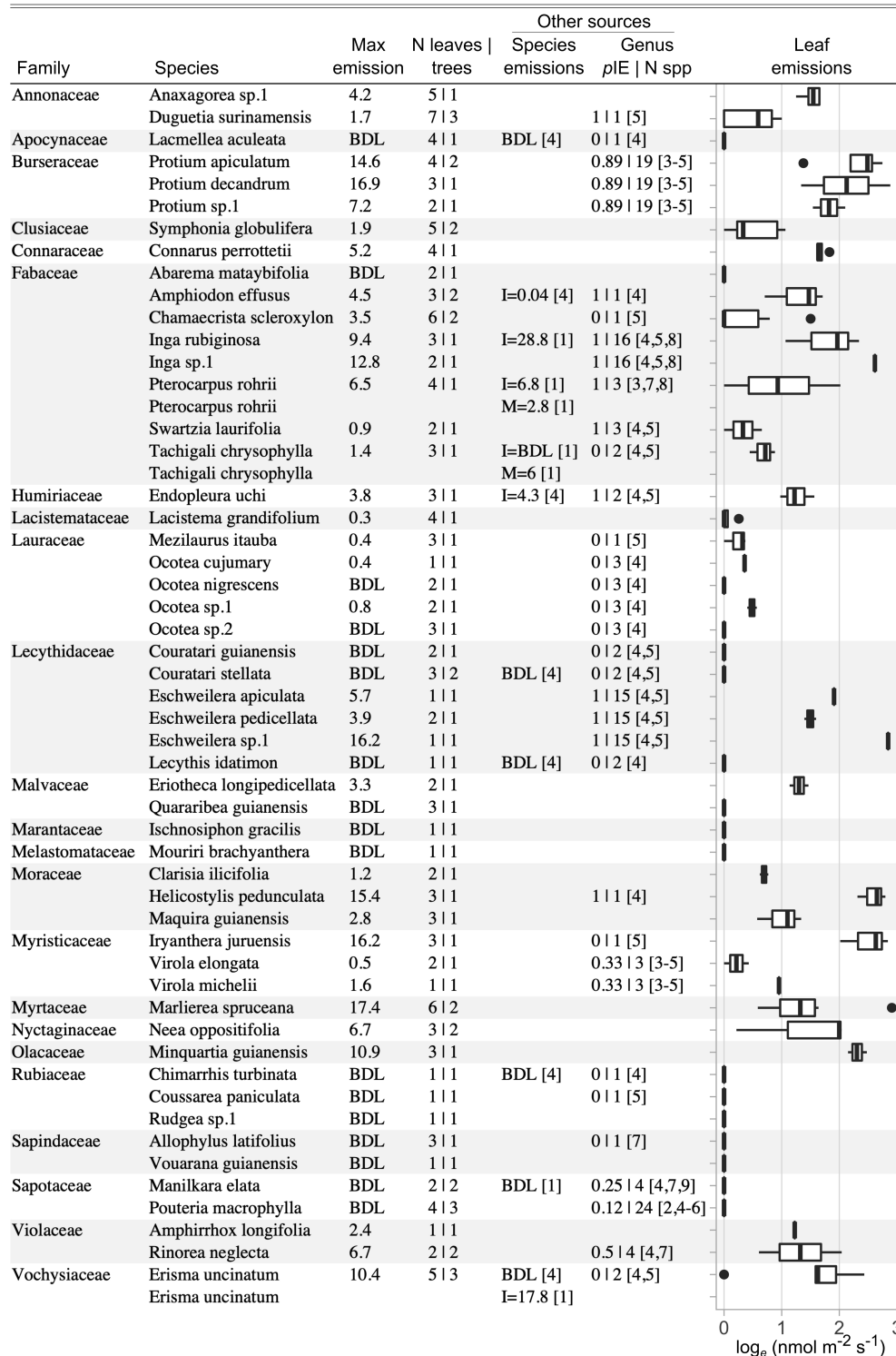
FIGURE 13 | Volatile isoprenoid emission rates from 52 tree species at an eastern Amazon site, the Tapajós National Forest, PA, Brazil. Emission rates are calculated from the end of a 210 s period of leaf illumination at 1000 PAR. Detectable emission rates were subsequently standardized to 30°C based on a standard temperature response curve. Max emission per species is provided (tabular, in \text{nmol}_M \text{m}^{-2}_{\text{leaf}} \text{s}^{-1} ), as well as the distributions of emissions from all leaf measurements (graphical, \log_e transformed). Validation measurements by GC-MS from this study and published estimates for isoprene (I) and monoterpenes (M) from a previous study at the same site are provided for shared species. Genus level data from literature is provided in units of proportion of measured species that emit isoprene (pIE) along with the number of species measured (N spp.). Numbered references: [1] Present study GC-MS validation measurements; [2] Bracho-Nunez et al. (2013); [3] Geron et al. (2002); [4] Harley et al. (2004); [5] Jardine et al. (2020a); [6] Klinger et al. (2002); [7] Klinger et al. (1998); [8] Taylor et al. (2018); [9] Varshney and Singh (2003).
