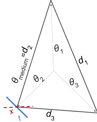
FIG. 8. Convention for coordinates systems. Top panel: TreeCorr internal variables and side length definitions as utilized in Eqs. (B1)–(B5), reproduced from [30]. Bottom panel: definition of distances of interest and shear projections ( t, \times ) relevant in the \Gamma_i(\theta_{\text{medium}}) and \langle M_{\text{ap}}(\theta_1, \theta_2, \theta_3) \rangle measurements. Notably, the reference scale \theta_{\text{medium}} is a side length, while the scales \theta_i ( i = 1, 2, 3 ) are radii from the triangle center.
