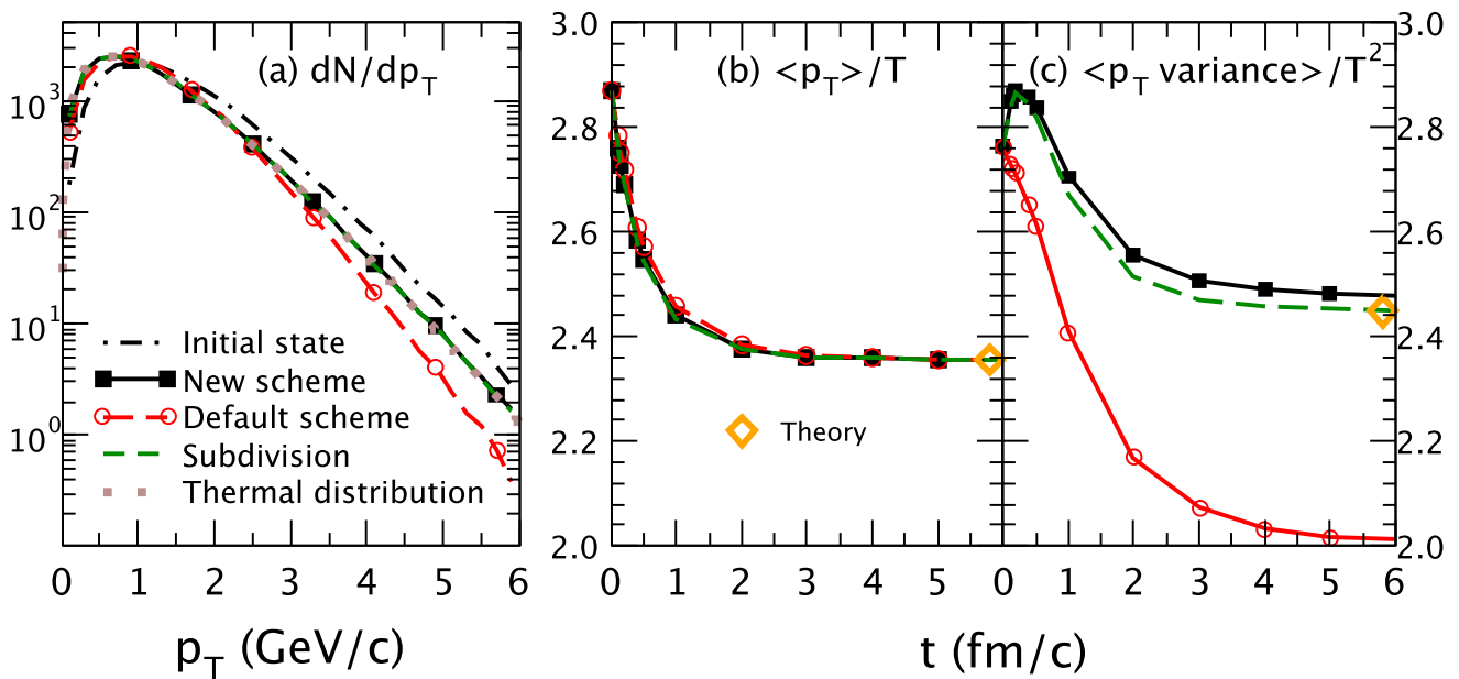
Fig. 19 (Color online) a The final p_T distribution, b time evolution of \langle p_T \rangle/T , and c time evolution of \langle p_T \text{ variance} \rangle/T^2 from ZPC from the default collision scheme (open circles) and the new collision scheme (filled squares) in comparison with parton subdivision results
