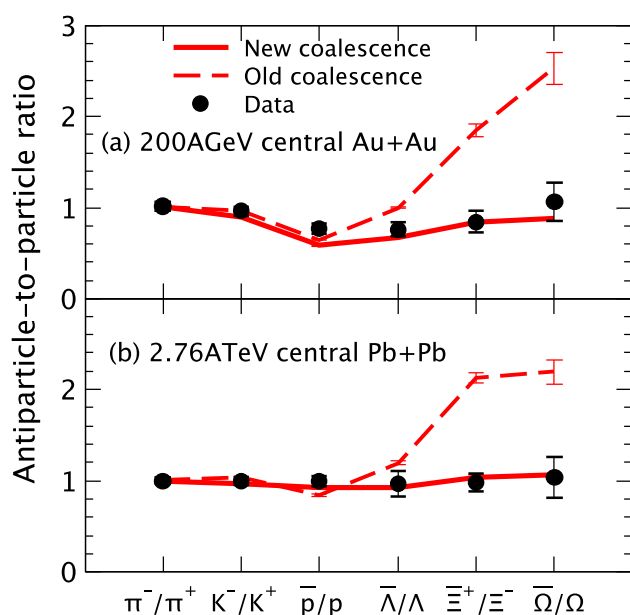
Fig. 5 (Color online) Antiparticle-to-particle ratios around mid-rapidity for a central Au+Au collisions at 200 GeV and b central Pb+Pb collisions at 2.76 TeV from the new (solid curves) and old (dashed curves) quark coalescence in comparison with the experimental data.
