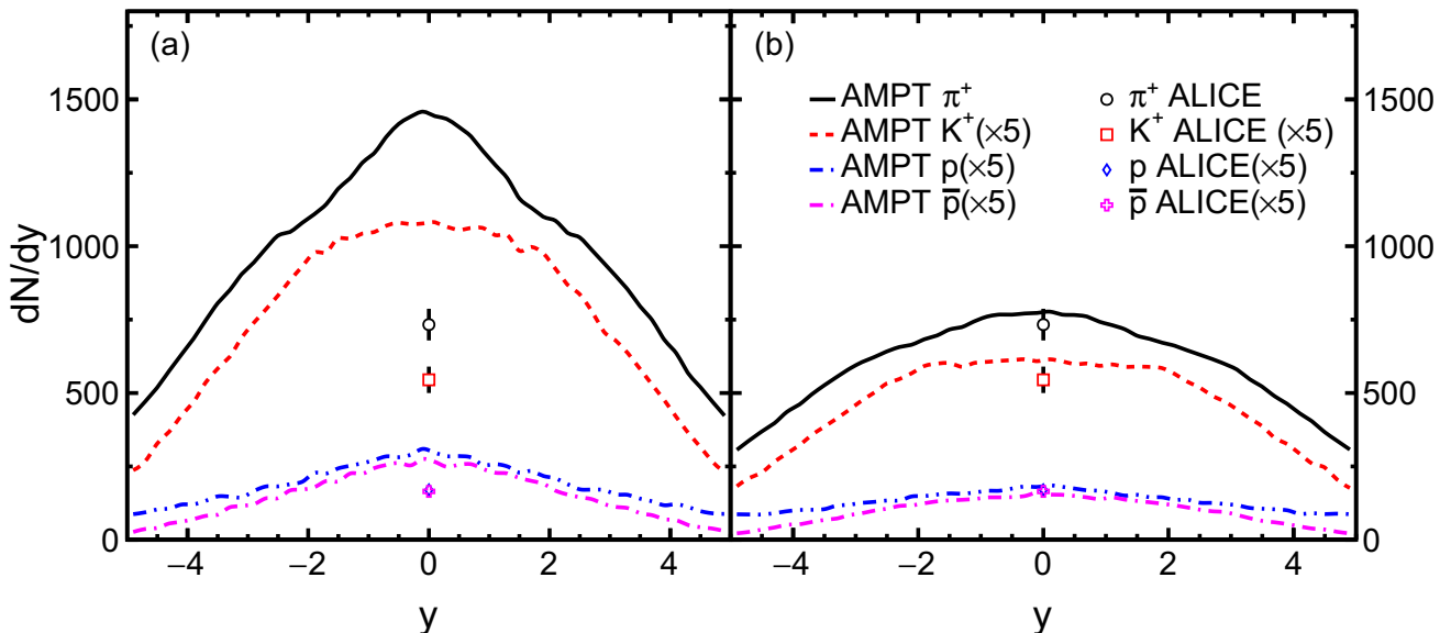
Fig. 9 (Color online) Identified particle rapidity distributions in 0–5% central Pb+Pb collisions at \sqrt{s_{NN}} = 2.76 TeV from the AMPT-SM model using the minijet cutoff a p_0^{pp}(s) or b p_0^{AA}(s) in comparison with the ALICE data [99, 101]
