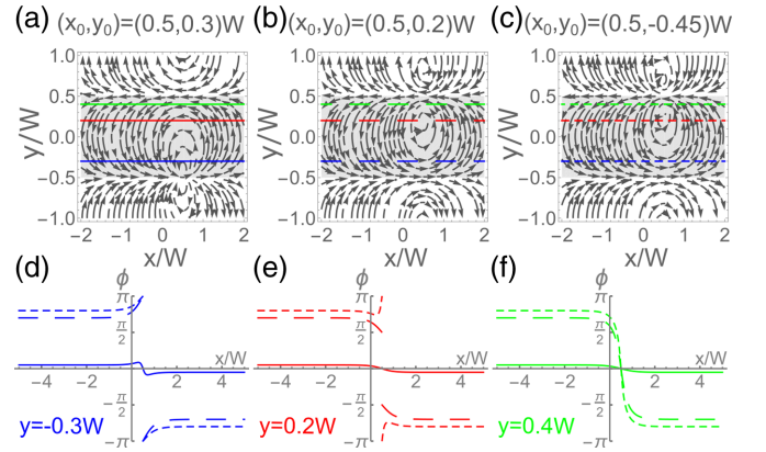
FIG. 2. A single vortex at position (x_0, y_0) tunneling from lower to the upper edge. (a)–(c) Gradient of the superconducting phase \nabla\phi . Note that mirror charges outside the sample (gray shaded) ensure no current outflux. (d)–(f) Principal branch of the phase \phi along the colored horizontal lines of panels (a)–(c) (same color and dashed code).
