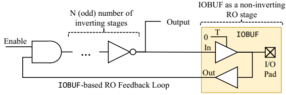
Fig. 1. Diagram of the proposed IOBUF-based RO design.
