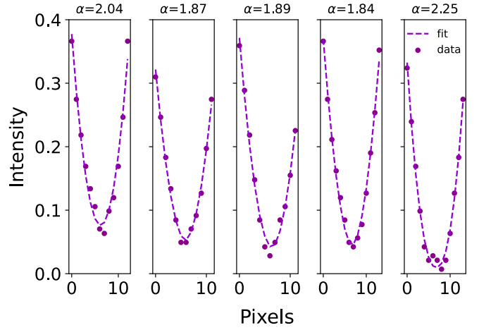
FIG. 8. A row of adjacent trap site profiles from the data shown in Fig. 2, where each site has been fit to a form a\rho^\alpha + b . The data were clipped above the 1/e intensity to ensure fitting to the lower order portions of the traps. It is clear that the experimentally observed radial profiles are nearly quadratic, rather than the quartic profiles expected for t_a = 0.287t_b with zero relative mask phase.
