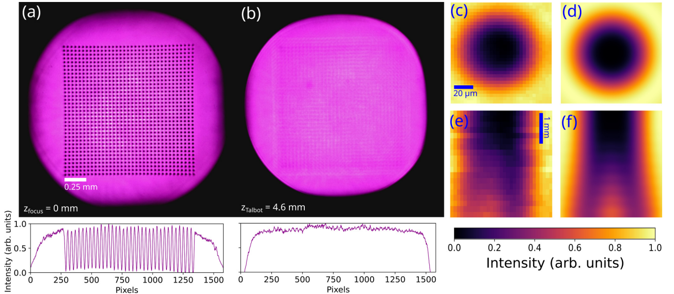
FIG. 3. Dark trap intensity profile with broadband, spatially multimode light. (a) The focal plane of traps imaged onto a CCD, formed with a 4f filtering system with a magnification of 1/10 , giving an array period of 43\ \mu\text{m} in the imaging plane. For the \lambda = 805\ \text{nm} light used, (b) the Talbot plane is located at z = 4.6\ \text{mm} , where the reimaged traps have been strongly suppressed. (c) and (e) show a single trap site with 808-nm multimode light projected on the focal plane and along the propagation plane intersecting \rho = 0 . For qualitative comparison, (d) and (f) show numerical simulations of the trap using coherent single mode light.
