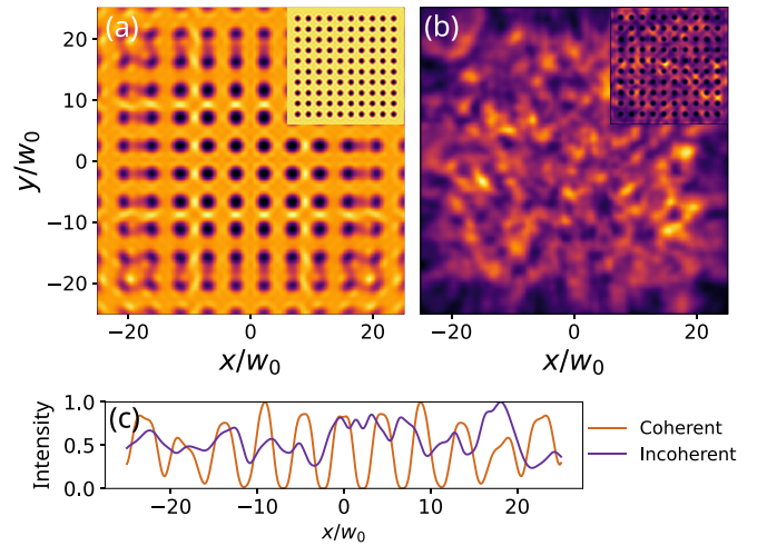
FIG. 7. Comparison of simulated Talbot plane trap formation for a 10 \times 10 dark aG array formed with (a) spatially coherent monochromatic light and (b) spectrally and spatially incoherent field. For the incoherent light, there are 21 frequency components spanning \Delta\lambda_{\text{FWHM}} = 3 nm, each with 200 Hermite-Gaussian modes with random phases. The insets show the the focal plane intensity. The plot axes are scaled to the best fit Gaussian waist, w_0 = 0.943a(f_2/f_1) . (c) Line profile comparison of a row of traps from (a) and (b), showing the washed out Talbot interference for the multimode light. For both simulations, \lambda_0 = 825 nm, d = 430 \mu\text{m} , and a = 100 \mu\text{m} , with a magnification of 1/100.
