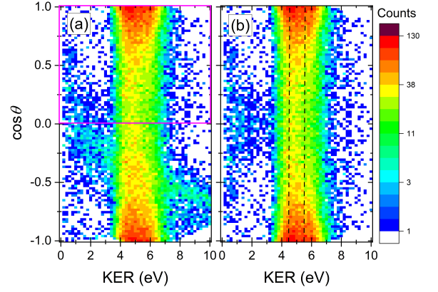
FIG. 2. The number of HCOOD^{2+} \rightarrow OH^+ + DCO^+ events (log scale) as a function of KER and \cos\theta , where \theta is the angle between the OH^+ fragment and the laser polarization. (a) The spectra after momentum conservation requirements and random coincidence subtraction, which still leaves contamination from another channel running diagonally through the lower half of the panel. (b) The same plot for the two-body channel after mirroring the \cos\theta > 0 data within the magenta rectangle onto the \cos\theta < 0 region of the plot. The two dashed lines at 4.4 eV and 5.6 eV mark the locations of the KER peaks of a two-Gaussian fit shown in Fig. 1.
