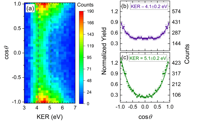
FIG. 9. (a) The number of \text{HCOOH}^{2+} \rightarrow \text{O}^+ + \text{H}_2\text{CO}^+ deoxygenation events (Eq. 3) as a function of KER and \cos \theta . The dashed vertical lines indicate the center of regions used to construct the angular distributions shown in the following panels. (b) Normalized yield of deoxygenation (Eq. 3) as a function of \cos \theta for KER within the range 4.1 \pm 0.2 eV. (c) The same plot, except for the higher 5.1 \pm 0.2 eV KER range. All of these angular distributions are obtained by reflecting the data about \cos \theta = 0 . In each plot, the solid lines represent the fit of the data to Eq. 13.
