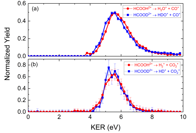
FIG. 4. Normalized yield as a function of KER for two-body breakup channels that involve bond rearrangement. (a) Water formation channels \text{H}_2\text{O}^+ + \text{CO}^+ (red circles) - Eq. 4 and \text{HDO}^+ + \text{CO}^+ (blue squares) - Eq. 11. (b) Hydrogen formation channels \text{H}_2^+ + \text{CO}_2^+ (red circles) - Eq. 5, and \text{HD}^+ + \text{CO}_2^+ (blue squares) Eq. 12. As with the other figures, the normalization sets the integral of each KER distribution to one.
