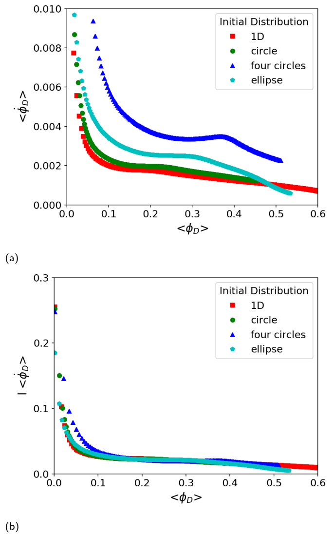
Fig. 12 (a) Reaction kinetics for different initial A homopolymer distributions in 2D. (b) The same data re-scaled by a characteristic interface length, l . The reaction rate for different mass distributions collapses when scaled in this way.
