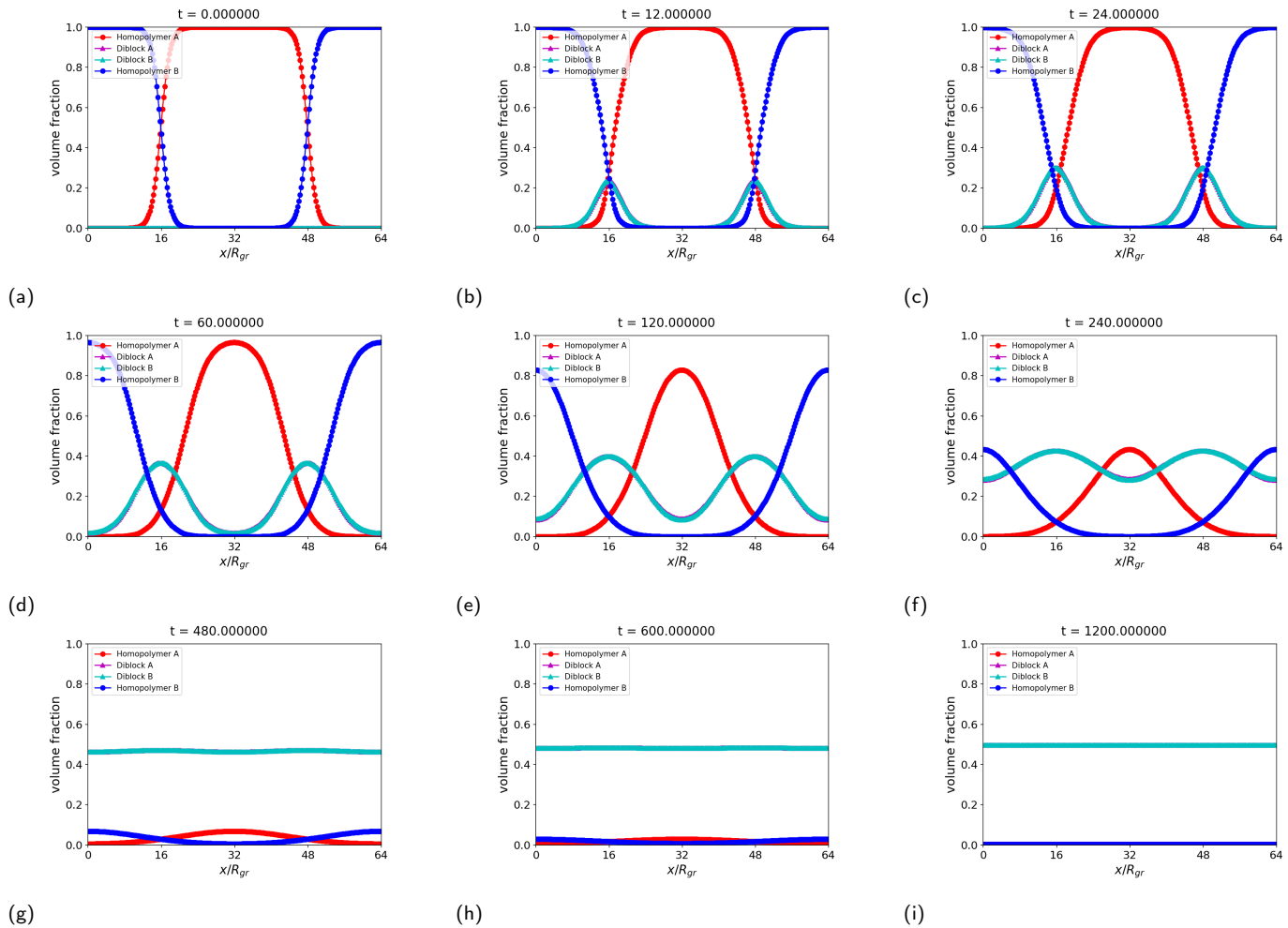
Fig. 4 Time evolution of volume fraction evolutions for a symmetric homopolymer blend undergoing an irreversible end-coupling reaction for Da_f = 0.3 , and \chi N_r = 3 . The copolymer builds up at the interface between the two homopolymers and diffuses into the bulk phases. As the homopolymer is slowly depleted, the system undergoes a phase transition into a DIS state.
