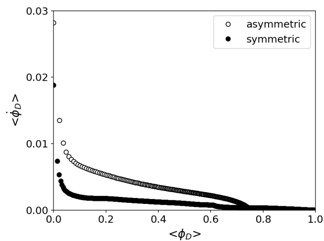
(a) reaction rate
