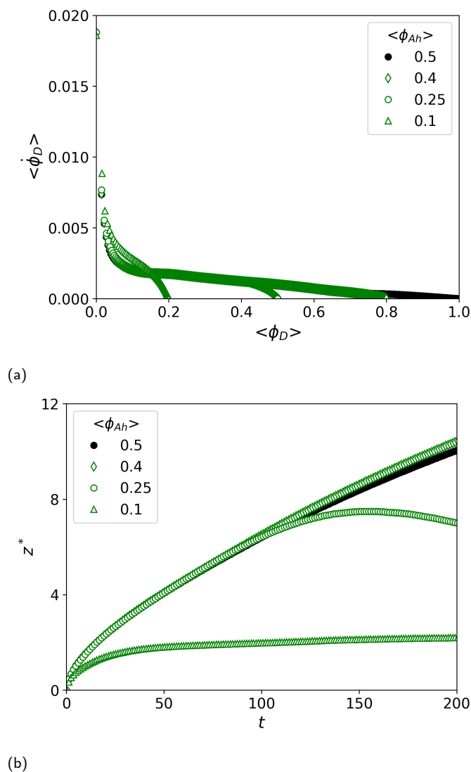
Fig. 13 Reaction kinetics (a) and interfacial excess (b) for an irreversible reaction of homopolymers with symmetric lengths but asymmetric compositions. The labels indicate the initial mean volume fraction of homopolymer A. While the initial kinetically limited and the eventual diffusion limited nature of the reaction is retained, a more asymmetric composition results in faster reactant depletion.
