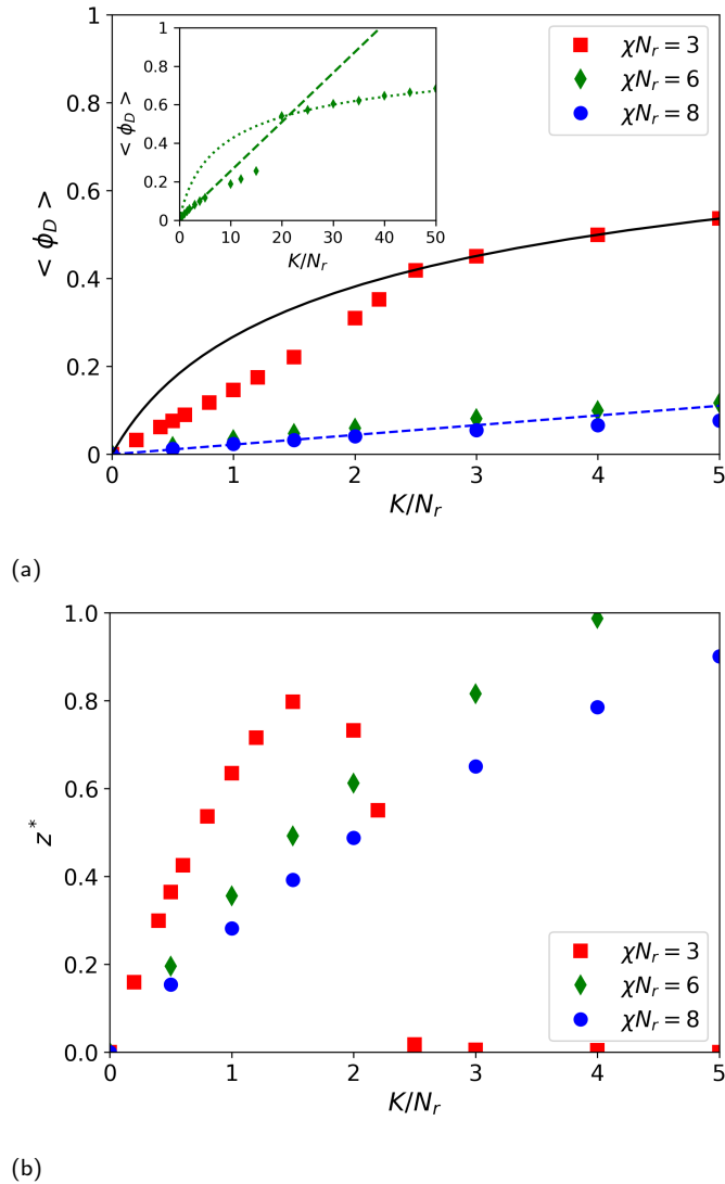
Fig. 11 Mean copolymer concentration (top) and interfacial excess (bottom) at equilibrium for a symmetric reversibly reacting blend for varying K/N_r and Da_f = 1 with a box size 32R_{gr} . The solid black line is obtained for a DIS system using Equation 26, while the blue dashed line is obtained for a 2\phi system using Equation 25 for \chi N_r = 8 . The inset shows the mean copolymer concentration for \chi N_r = 6 for a wider range of K/N_r . The green dashed line is obtained for a 2\phi system using Equation 25 while the green dotted line is obtained for a LAM system using Equation 27.
