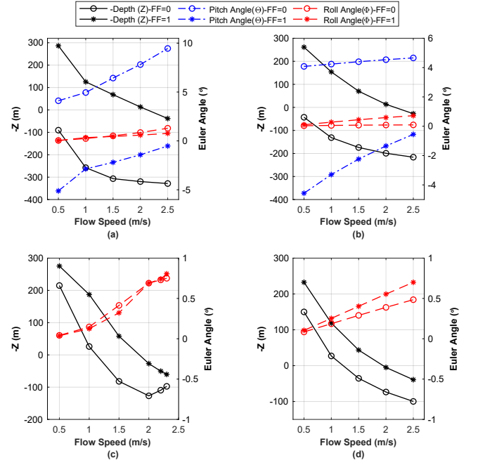
Fig. 4. Operating range assessment for (a) homogeneous flow speeds, (b) shear flow speeds, (c) homogeneous flow speeds ensuring the pitch angle is driven towards zero, and (d) shear flow speed ensuring the pitch angle is driven towards zero.
