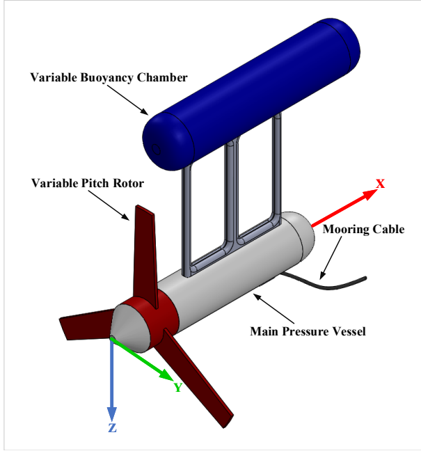
Fig. 1. Schematic of the numerically simulated buoyancy controlled ocean current turbine.
