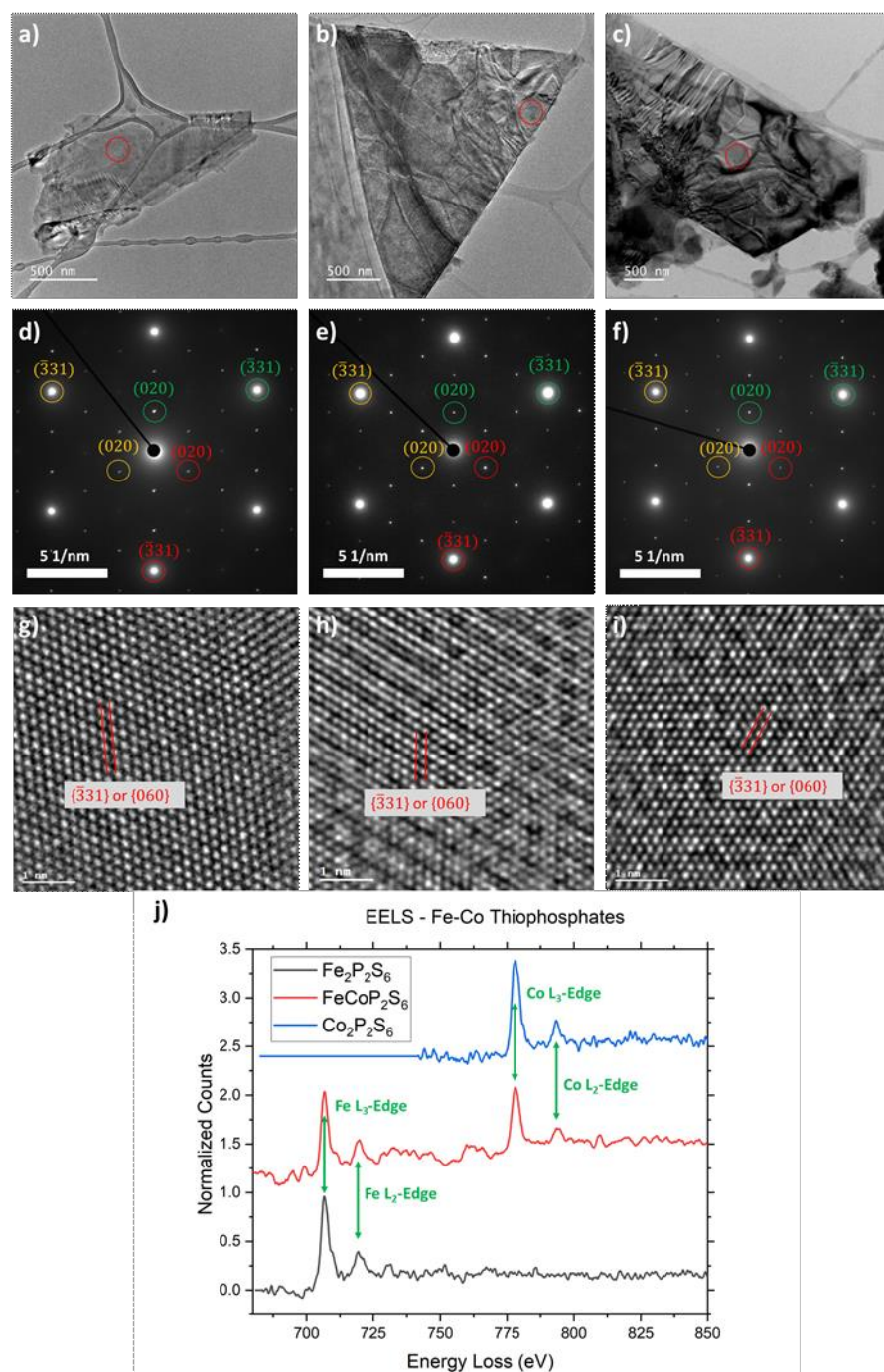
Figure 2. a-c) Low resolution TEM bright-field images for Fe 2 P 2 S 6 , FeCoP 2 S 6 , and Co 2 P 2 S 6 , respectively. The red circle indicates the location of the selected area electron diffraction (SAED) aperture where SAED patterns are taken. d-f) SAED patterns for Fe 2 P 2 S 6 , FeCoP 2 S 6 , and Co 2 P 2 S 6 , respectively. SAED pattern taken along the c *-axis which is nearly parallel to the -z -zone axis. The SAED pattern exhibits the presence of 120°-twins along the out-of-plane direction. g-i) High resolution TEM (HRTEM) images of Fe 2 P 2 S 6 , FeCoP 2 S 6 , and Co 2 P 2 S 6 , respectively with the { \bar{3}31 } or {060} planes indicated. j) Core-loss EELS for Fe 2 P 2 S 6 , FeCoP 2 S 6 , and Co 2 P 2 S 6 with the Fe-L Edges and Co-L Edges indicated. The atomic percentage indicating the ratio of Fe and Co are shown.
