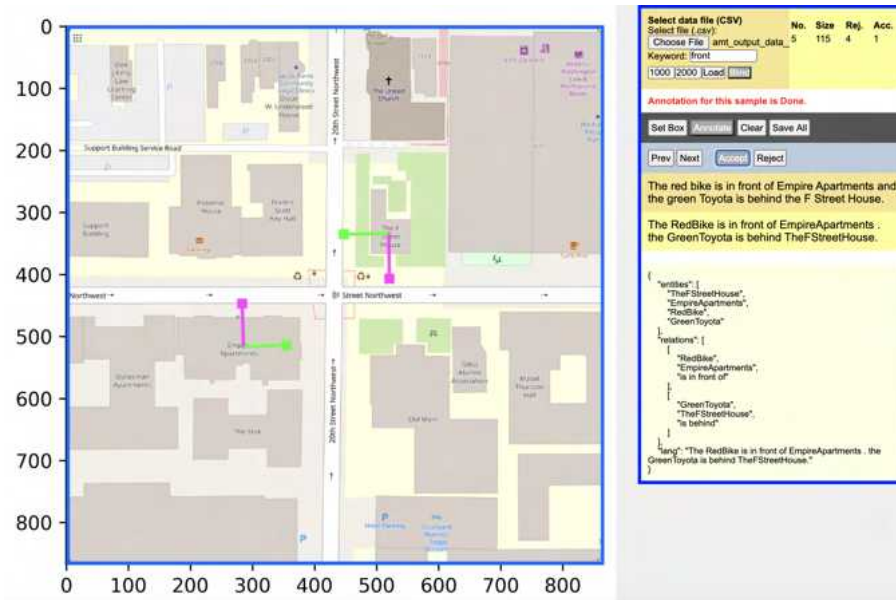
Fig. 12: The FoR annotator GUI interface. The FoR consists of a front (purple) and right (green) vector. The target objects are not shown, and the annotator only has access to the spatial language description, and the map image. This mimics the situation faced by the robot in our task.
