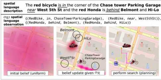
Fig. 2: We consider a spatial language description as an observation O_R , which is a set of (f, r, \gamma) tuples, obtained through parsing the input language. We propose an observation model that incorporates the spatial information in O_R into the robot’s belief about target locations, which benefits subsequent object search performance.
