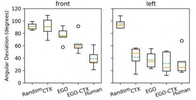
Fig. 5: FoR prediction results. The solid orange line shows the median, and the dotted green line shows the mean. The circles are outliers. Lower is better.
